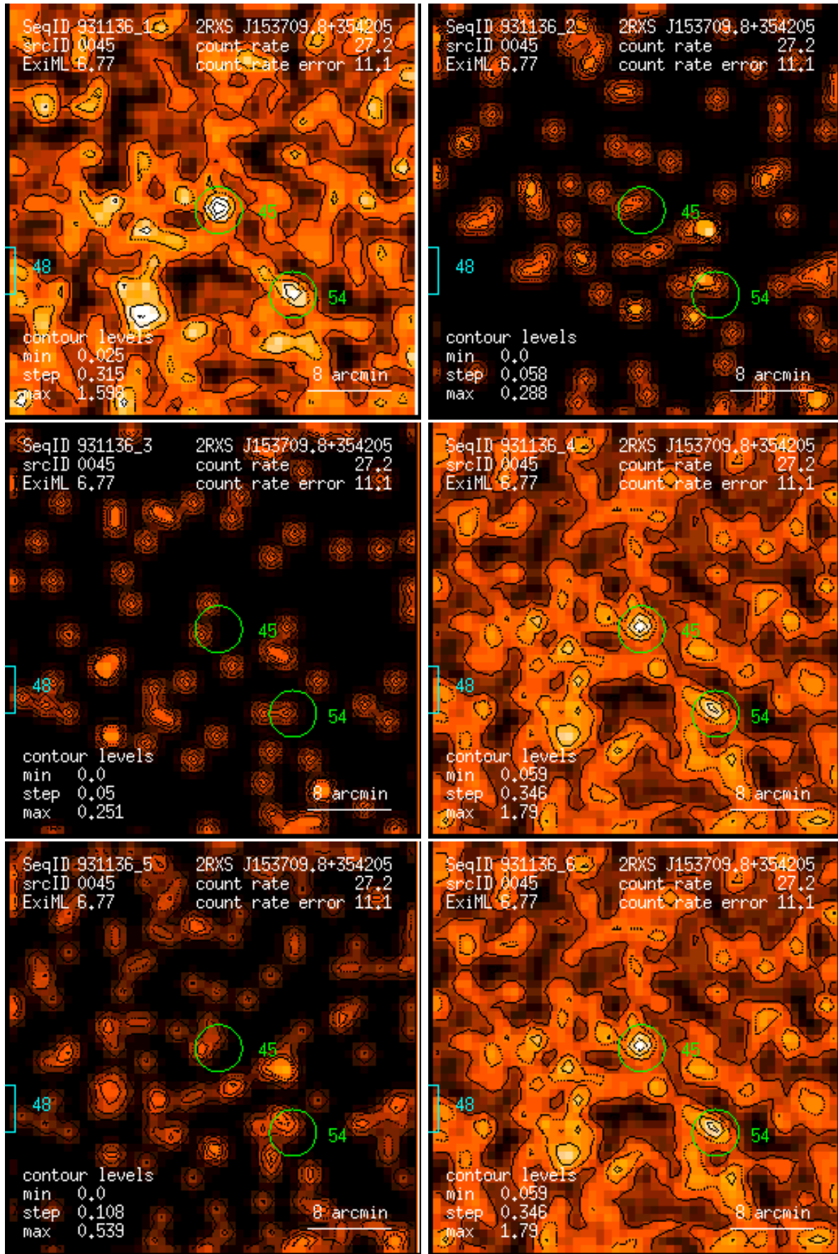
Figure 45: RASS 931136: detection 0045: band rate images, Gaussian filter: (1) PSPC channels 11 – 41, (2) 52 – 90, (3) 91 – 201, (4) 11 – 235, (5) 52 – 201, (6) 11 – 201. Broad band rates in counts/ks. Band rate contour levels in counts/ks/arcmin 2 .
