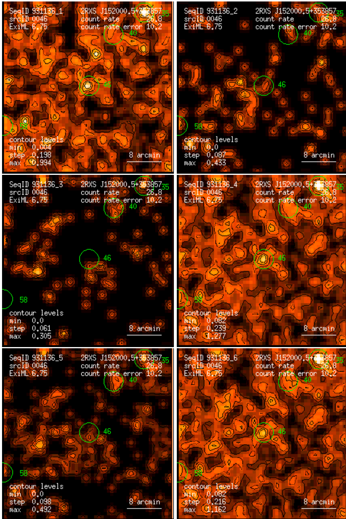
Figure 46: RASS 931136: detection 0046: band rate images, Gaussian filter: (1) PSPC channels 11 – 41, (2) 52 – 90, (3) 91 – 201, (4) 11 – 235, (5) 52 – 201, (6) 11 – 201. Broad band rates in counts/ks. Band rate contour levels in counts/ks/arcmin 2 .
