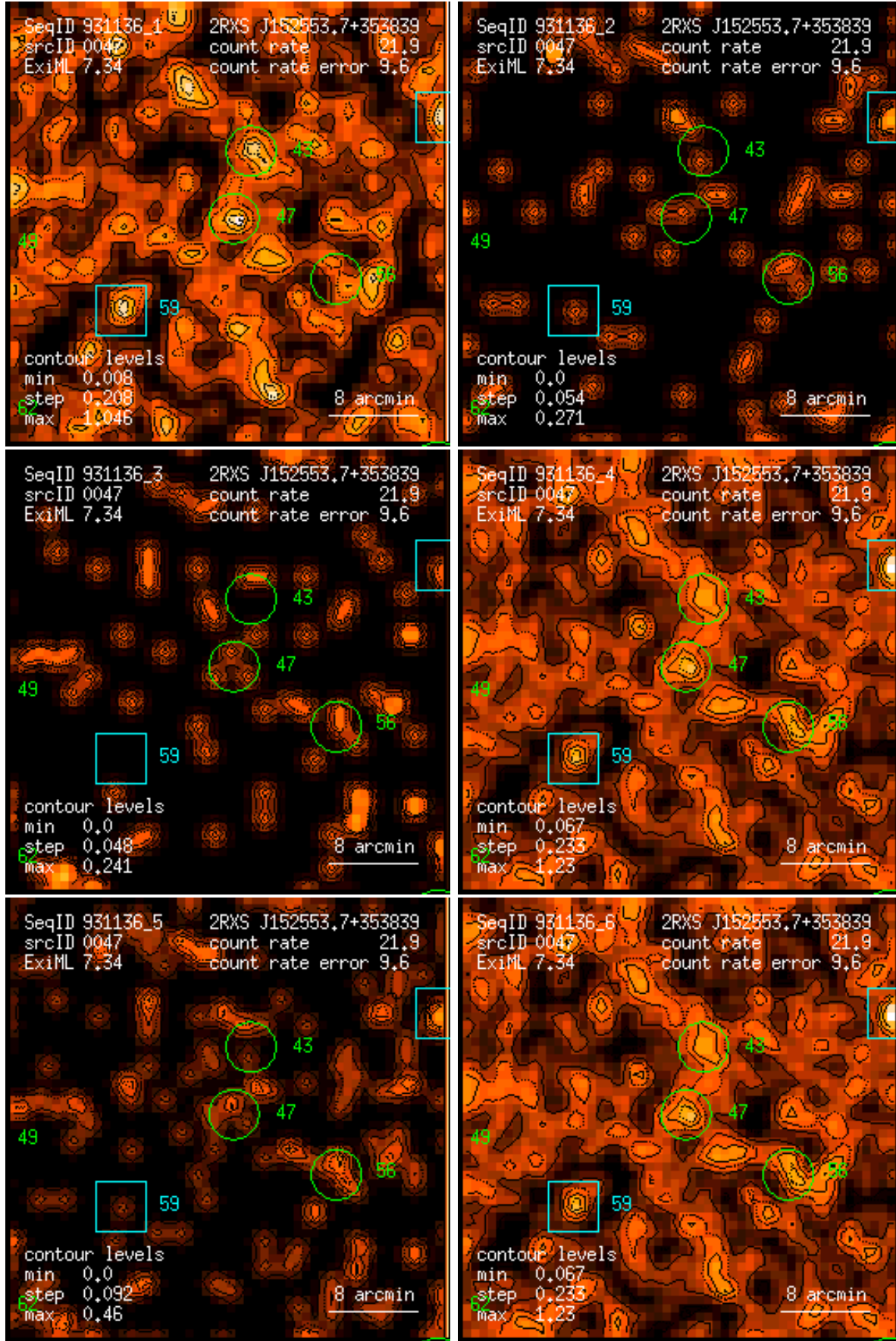
Figure 47: RASS 931136: detection 0047: band rate images, Gaussian filter: (1) PSPC channels 11 – 41, (2) 52 – 90, (3) 91 – 201, (4) 11 – 235, (5) 52 – 201, (6) 11 – 201. Broad band rates in counts/ks. Band rate contour levels in counts/ks/arcmin 2 .
