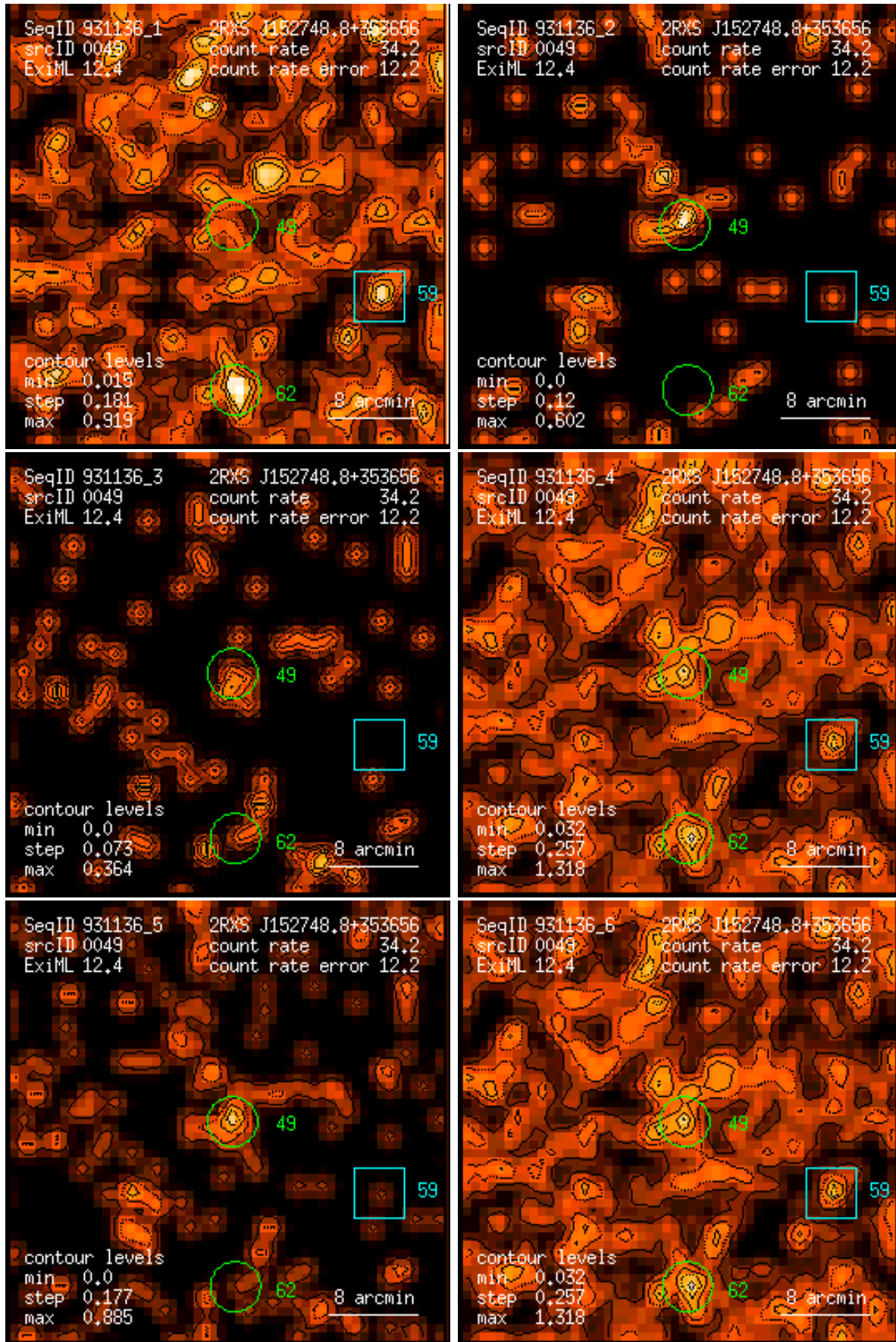
Figure 49: RASS 931136: detection 0049: band rate images, Gaussian filter: (1) PSPC channels 11 – 41, (2) 52 – 90, (3) 91 – 201, (4) 11 – 235, (5) 52 – 201, (6) 11 – 201. Broad band rates in counts/ks. Band rate contour levels in counts/ks/arcmin 2 .
