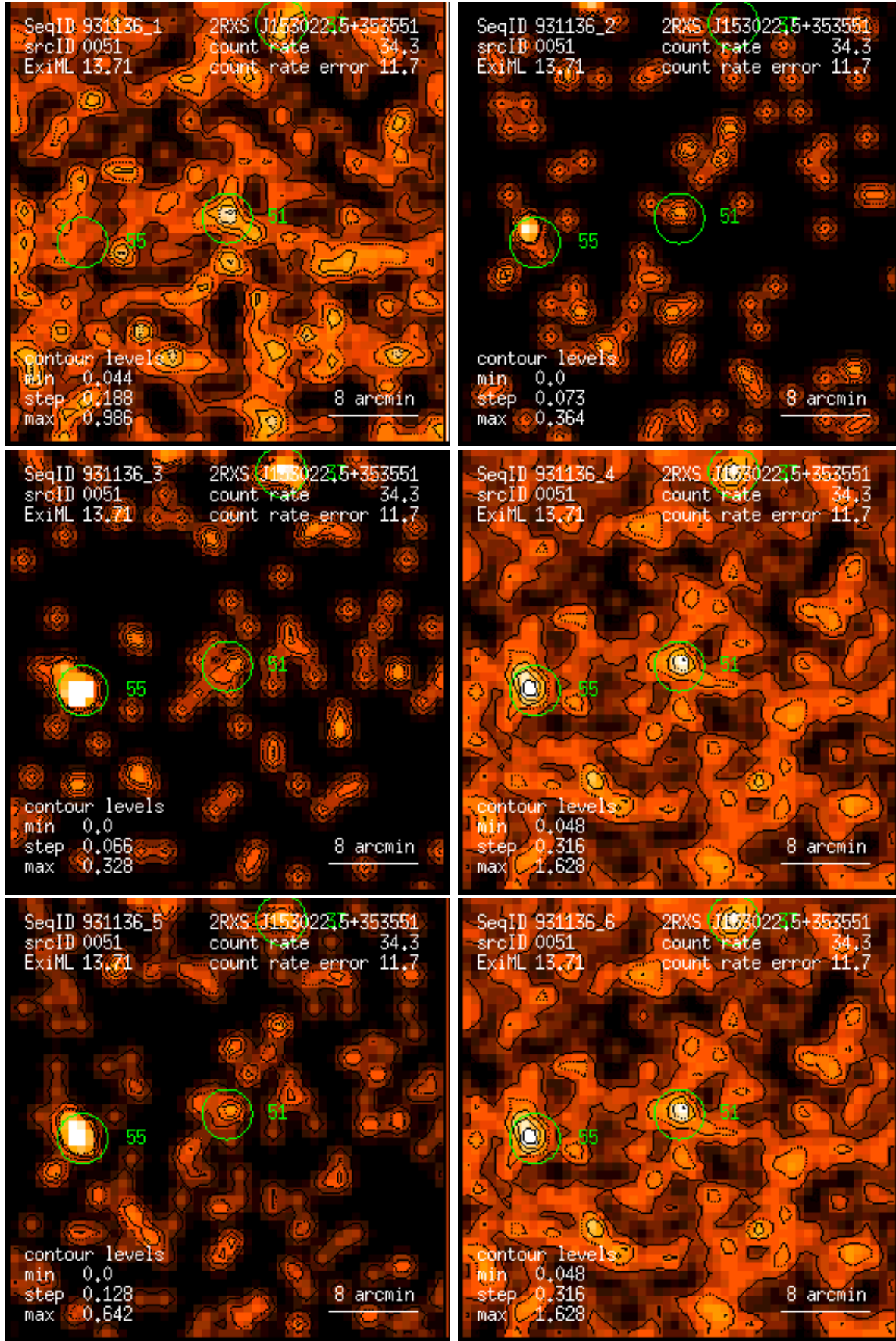
Figure 51: RASS 931136: detection 0051: band rate images, Gaussian filter: (1) PSPC channels 11 – 41, (2) 52 – 90, (3) 91 – 201, (4) 11 – 235, (5) 52 – 201, (6) 11 – 201. Broad band rates in counts/ks. Band rate contour levels in counts/ks/arcmin 2 .
