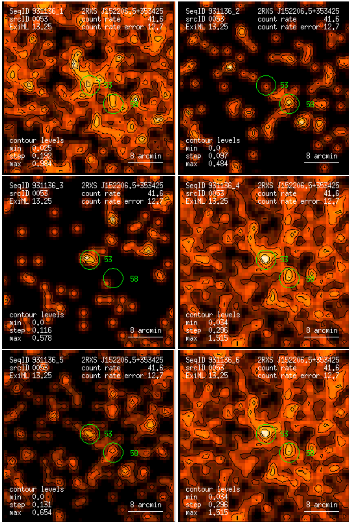
Figure 53: RASS 931136: detection 0053: band rate images, Gaussian filter: (1) PSPC channels 11 – 41, (2) 52 – 90, (3) 91 – 201, (4) 11 – 235, (5) 52 – 201, (6) 11 – 201. Broad band rates in counts/ks. Band rate contour levels in counts/ks/arcmin 2 .
