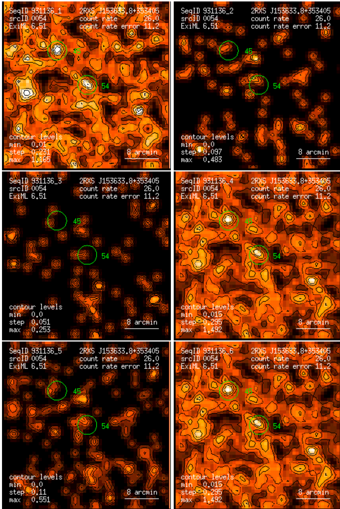
Figure 54: RASS 931136: detection 0054: band rate images, Gaussian filter: (1) PSPC channels 11 – 41, (2) 52 – 90, (3) 91 – 201, (4) 11 – 235, (5) 52 – 201, (6) 11 – 201. Broad band rates in counts/ks. Band rate contour levels in counts/ks/arcmin 2 .
