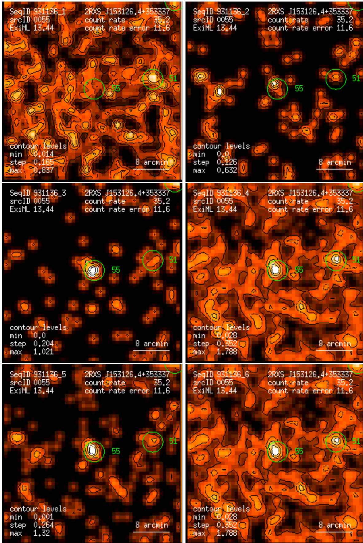
Figure 55: RASS 931136: detection 0055: band rate images, Gaussian filter: (1) PSPC channels 11 – 41, (2) 52 – 90, (3) 91 – 201, (4) 11 – 235, (5) 52 – 201, (6) 11 – 201. Broad band rates in counts/ks. Band rate contour levels in counts/ks/arcmin 2 .
