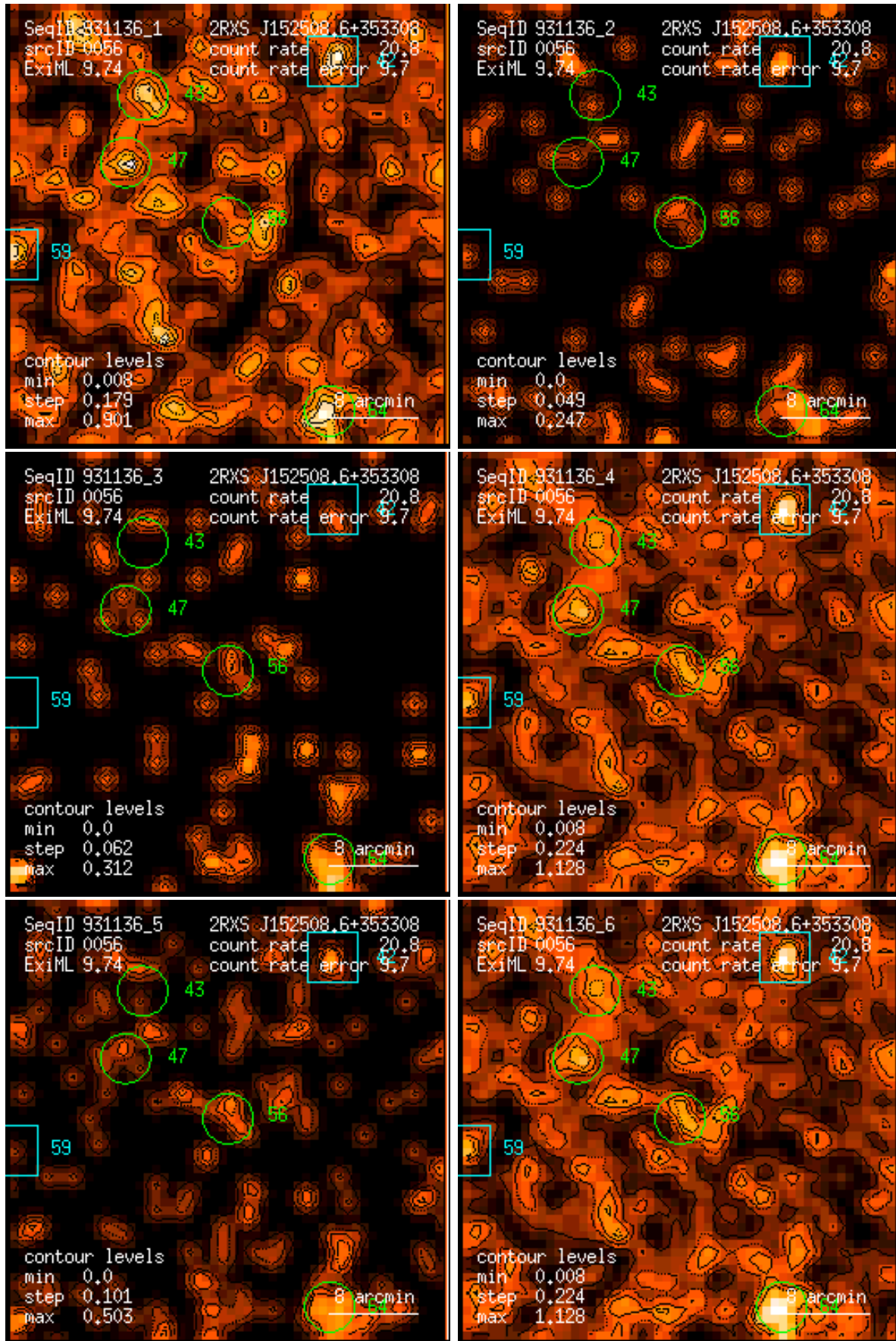
Figure 56: RASS 931136: detection 0056: band rate images, Gaussian filter: (1) PSPC channels 11 – 41, (2) 52 – 90, (3) 91 – 201, (4) 11 – 235, (5) 52 – 201, (6) 11 – 201. Broad band rates in counts/ks. Band rate contour levels in counts/ks/arcmin 2 .
