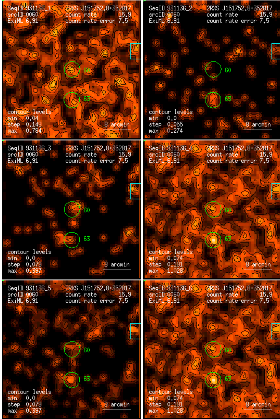
Figure 60: RASS 931136: detection 0060: band rate images, Gaussian filter: (1) PSPC channels 11 – 41, (2) 52 – 90, (3) 91 – 201, (4) 11 – 235, (5) 52 – 201, (6) 11 – 201. Broad band rates in counts/ks. Band rate contour levels in counts/ks/arcmin 2 .
