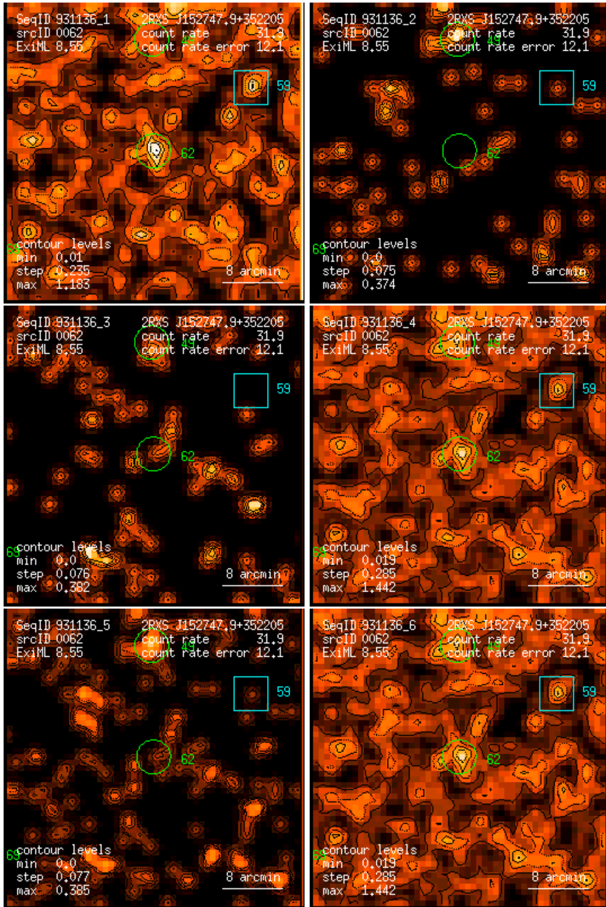
Figure 62: RASS 931136: detection 0062: band rate images, Gaussian filter: (1) PSPC channels 11 – 41, (2) 52 – 90, (3) 91 – 201, (4) 11 – 235, (5) 52 – 201, (6) 11 – 201. Broad band rates in counts/ks. Band rate contour levels in counts/ks/arcmin 2 .
