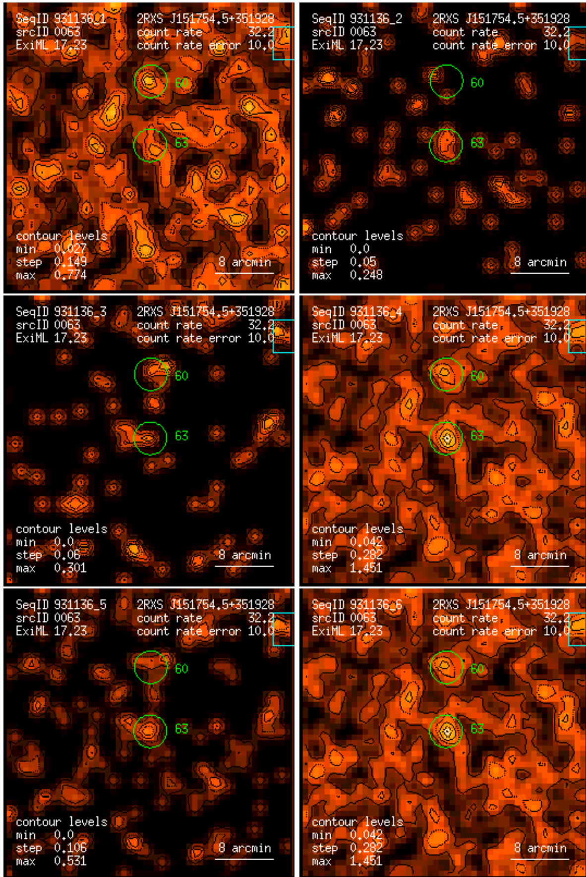
Figure 63: RASS 931136: detection 0063: band rate images, Gaussian filter: (1) PSPC channels 11 – 41, (2) 52 – 90, (3) 91 – 201, (4) 11 – 235, (5) 52 – 201, (6) 11 – 201. Broad band rates in counts/ks. Band rate contour levels in counts/ks/arcmin 2 .
