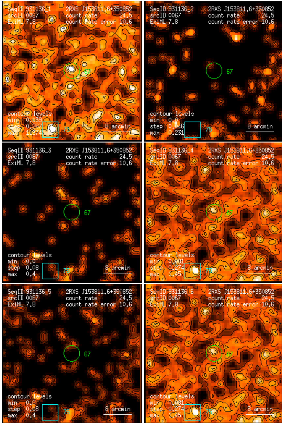
Figure 67: RASS 931136: detection 0067: band rate images, Gaussian filter: (1) PSPC channels 11 – 41, (2) 52 – 90, (3) 91 – 201, (4) 11 – 235, (5) 52 – 201, (6) 11 – 201. Broad band rates in counts/ks. Band rate contour levels in counts/ks/arcmin 2 .
