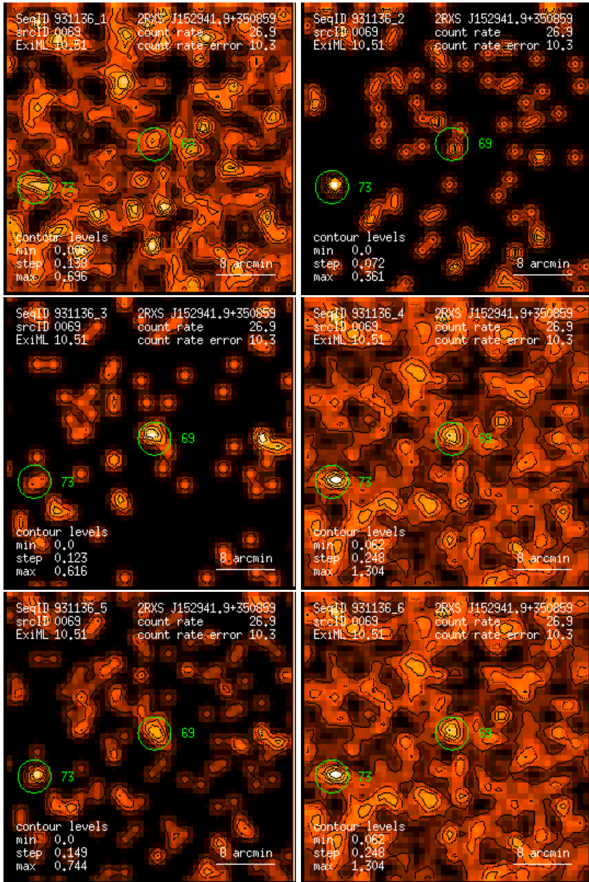
Figure 69: RASS 931136: detection 0069: band rate images, Gaussian filter: (1) PSPC channels 11 – 41, (2) 52 – 90, (3) 91 – 201, (4) 11 – 235, (5) 52 – 201, (6) 11 – 201. Broad band rates in counts/ks. Band rate contour levels in counts/ks/arcmin 2 .
