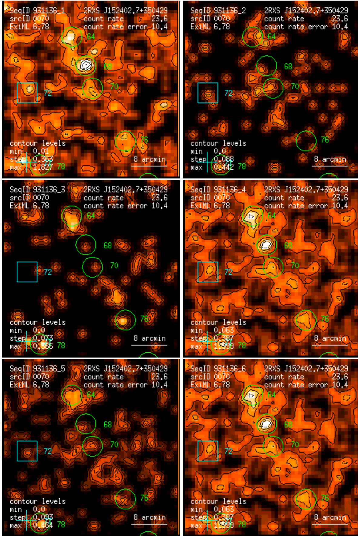
Figure 70: RASS 931136: detection 0070: band rate images, Gaussian filter: (1) PSPC channels 11 – 41, (2) 52 – 90, (3) 91 – 201, (4) 11 – 235, (5) 52 – 201, (6) 11 – 201. Broad band rates in counts/ks. Band rate contour levels in counts/ks/arcmin 2 .
