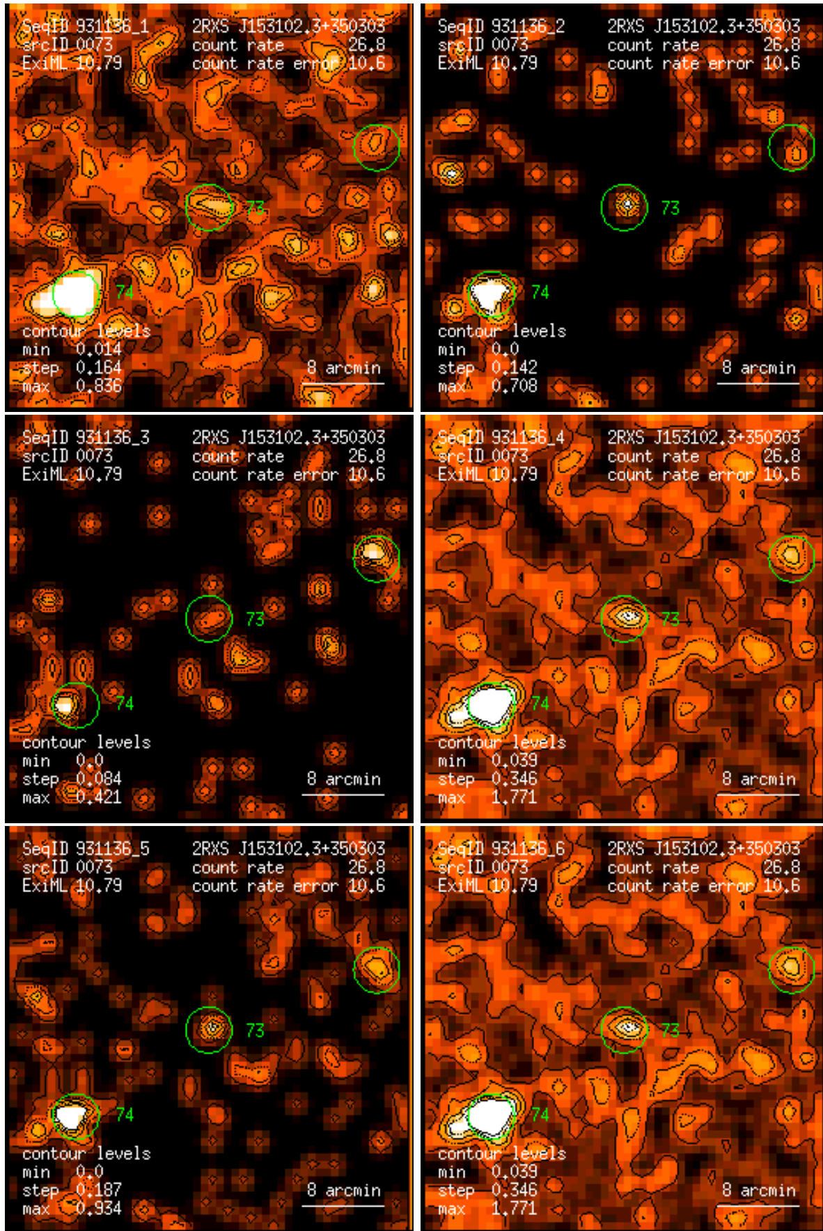
Figure 73: RASS 931136: detection 0073: band rate images, Gaussian filter: (1) PSPC channels 11 – 41, (2) 52 – 90, (3) 91 – 201, (4) 11 – 235, (5) 52 – 201, (6) 11 – 201. Broad band rates in counts/ks. Band rate contour levels in counts/ks/arcmin 2 .
