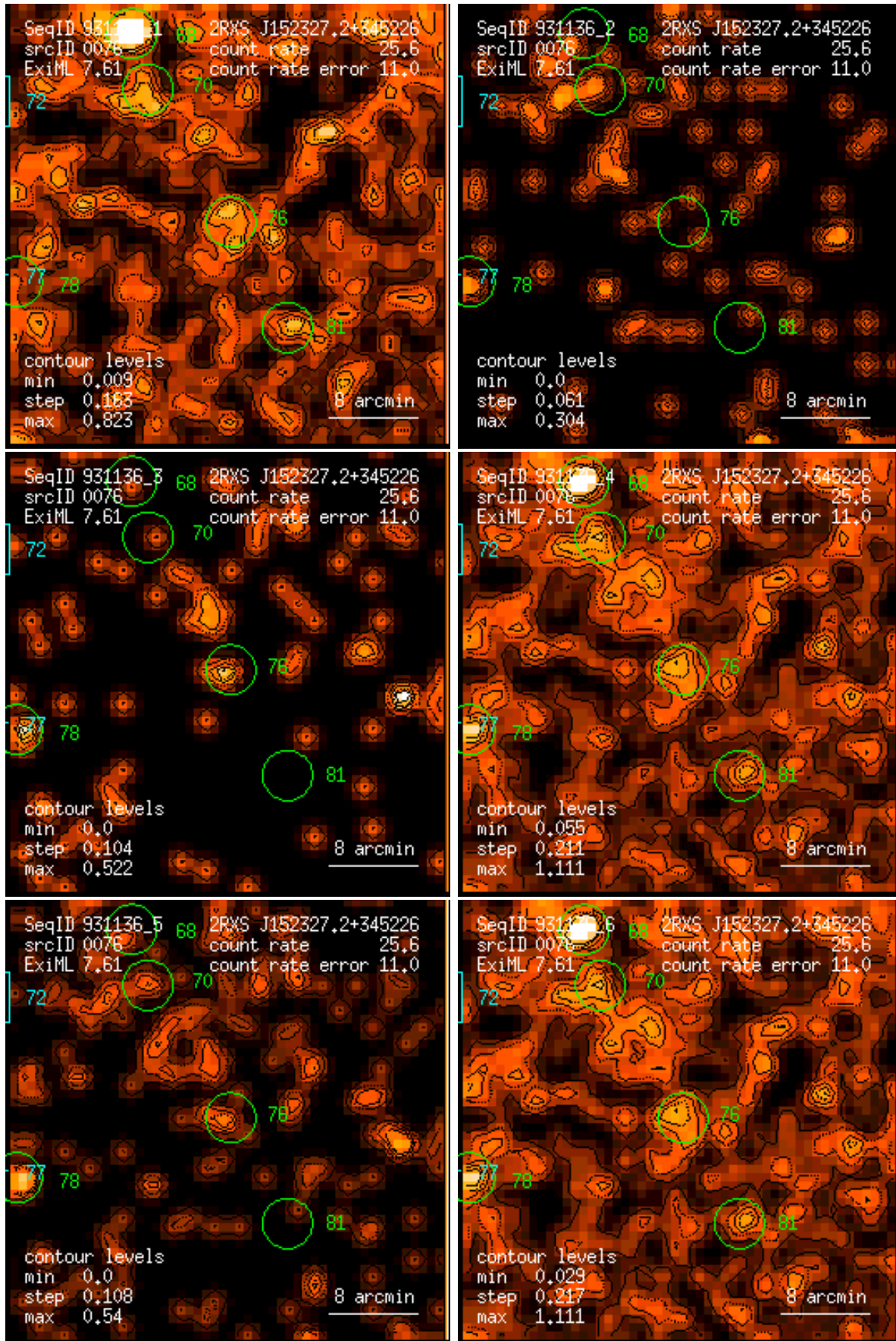
Figure 76: RASS 931136: detection 0076: band rate images, Gaussian filter: (1) PSPC channels 11 – 41, (2) 52 – 90, (3) 91 – 201, (4) 11 – 235, (5) 52 – 201, (6) 11 – 201. Broad band rates in counts/ks. Band rate contour levels in counts/ks/arcmin 2 .
