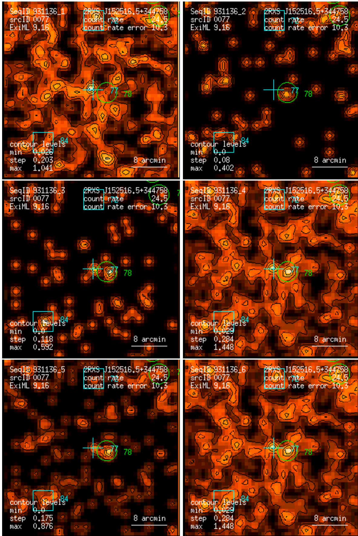
Figure 77: RASS 931136: detection 0077: band rate images, Gaussian filter: (1) PSPC channels 11 – 41, (2) 52 – 90, (3) 91 – 201, (4) 11 – 235, (5) 52 – 201, (6) 11 – 201. Broad band rates in counts/ks. Band rate contour levels in counts/ks/arcmin 2 .
