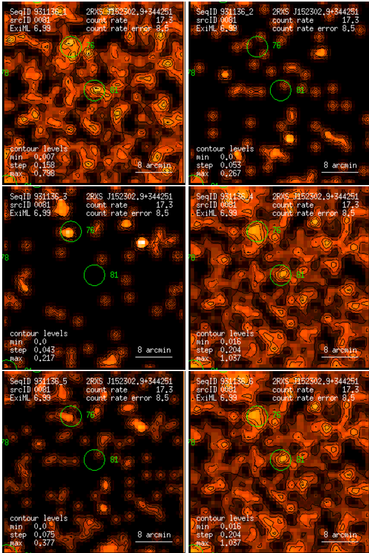
Figure 81: RASS 931136: detection 0081: band rate images, Gaussian filter: (1) PSPC channels 11 – 41, (2) 52 – 90, (3) 91 – 201, (4) 11 – 235, (5) 52 – 201, (6) 11 – 201. Broad band rates in counts/ks. Band rate contour levels in counts/ks/arcmin 2 .
