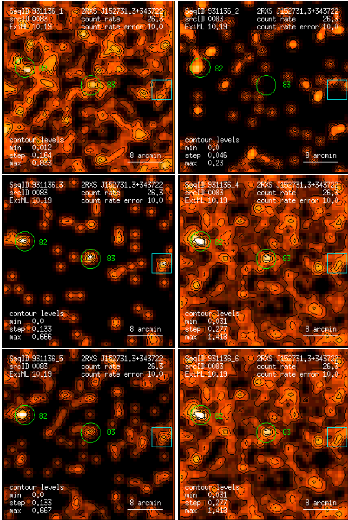
Figure 83: RASS 931136: detection 0083: band rate images, Gaussian filter: (1) PSPC channels 11 – 41, (2) 52 – 90, (3) 91 – 201, (4) 11 – 235, (5) 52 – 201, (6) 11 – 201. Broad band rates in counts/ks. Band rate contour levels in counts/ks/arcmin 2 .
