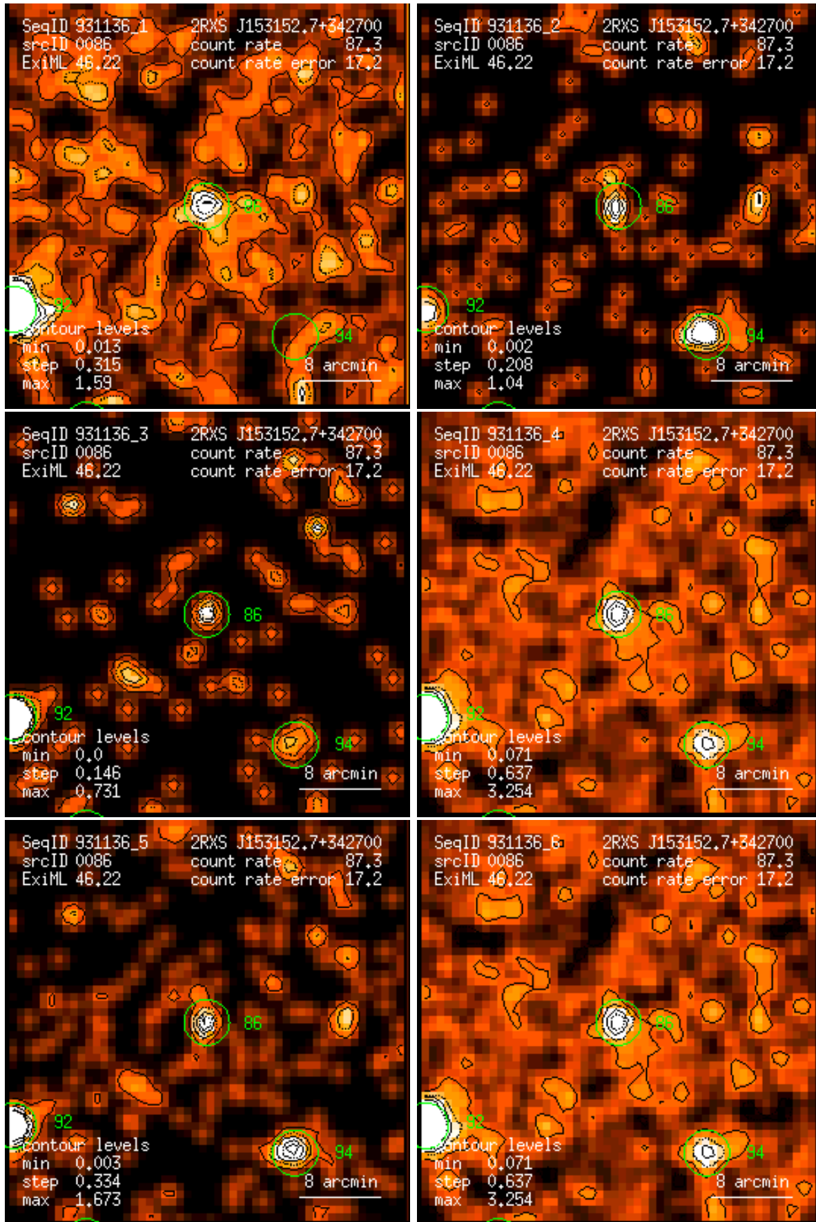
Figure 86: RASS 931136: detection 0086: band rate images, Gaussian filter: (1) PSPC channels 11 – 41, (2) 52 – 90, (3) 91 – 201, (4) 11 – 235, (5) 52 – 201, (6) 11 – 201. Broad band rates in counts/ks. Band rate contour levels in counts/ks/arcmin 2 .
