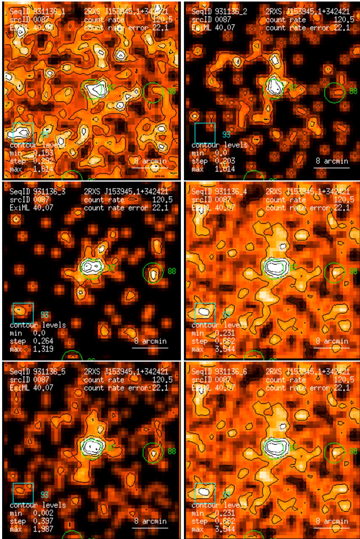
Figure 87: RASS 931136: detection 0087: band rate images, Gaussian filter: (1) PSPC channels 11 – 41, (2) 52 – 90, (3) 91 – 201, (4) 11 – 235, (5) 52 – 201, (6) 11 – 201. Broad band rates in counts/ks. Band rate contour levels in counts/ks/arcmin 2 .
