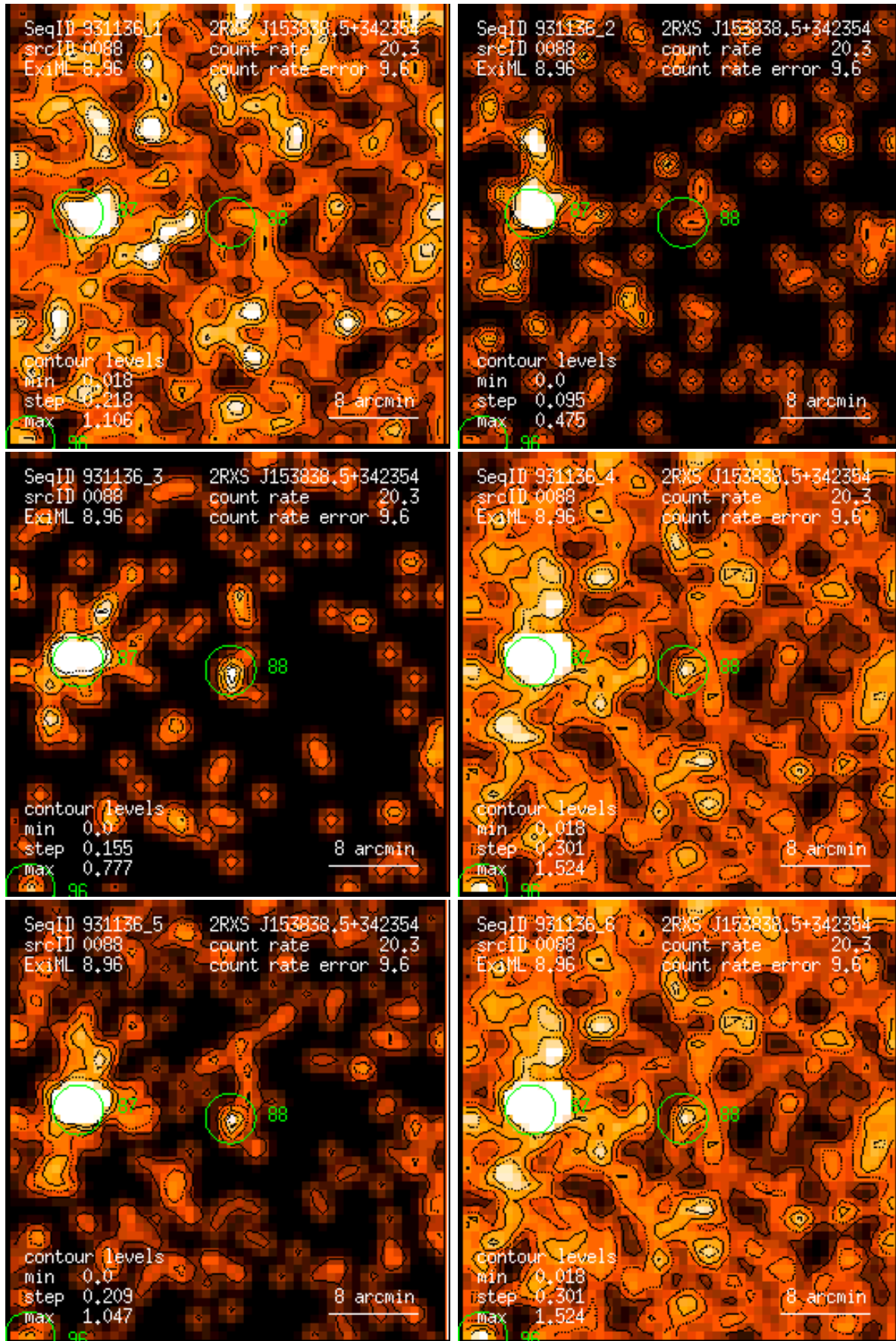
Figure 88: RASS 931136: detection 0088: band rate images, Gaussian filter: (1) PSPC channels 11 – 41, (2) 52 – 90, (3) 91 – 201, (4) 11 – 235, (5) 52 – 201, (6) 11 – 201. Broad band rates in counts/ks. Band rate contour levels in counts/ks/arcmin 2 .
