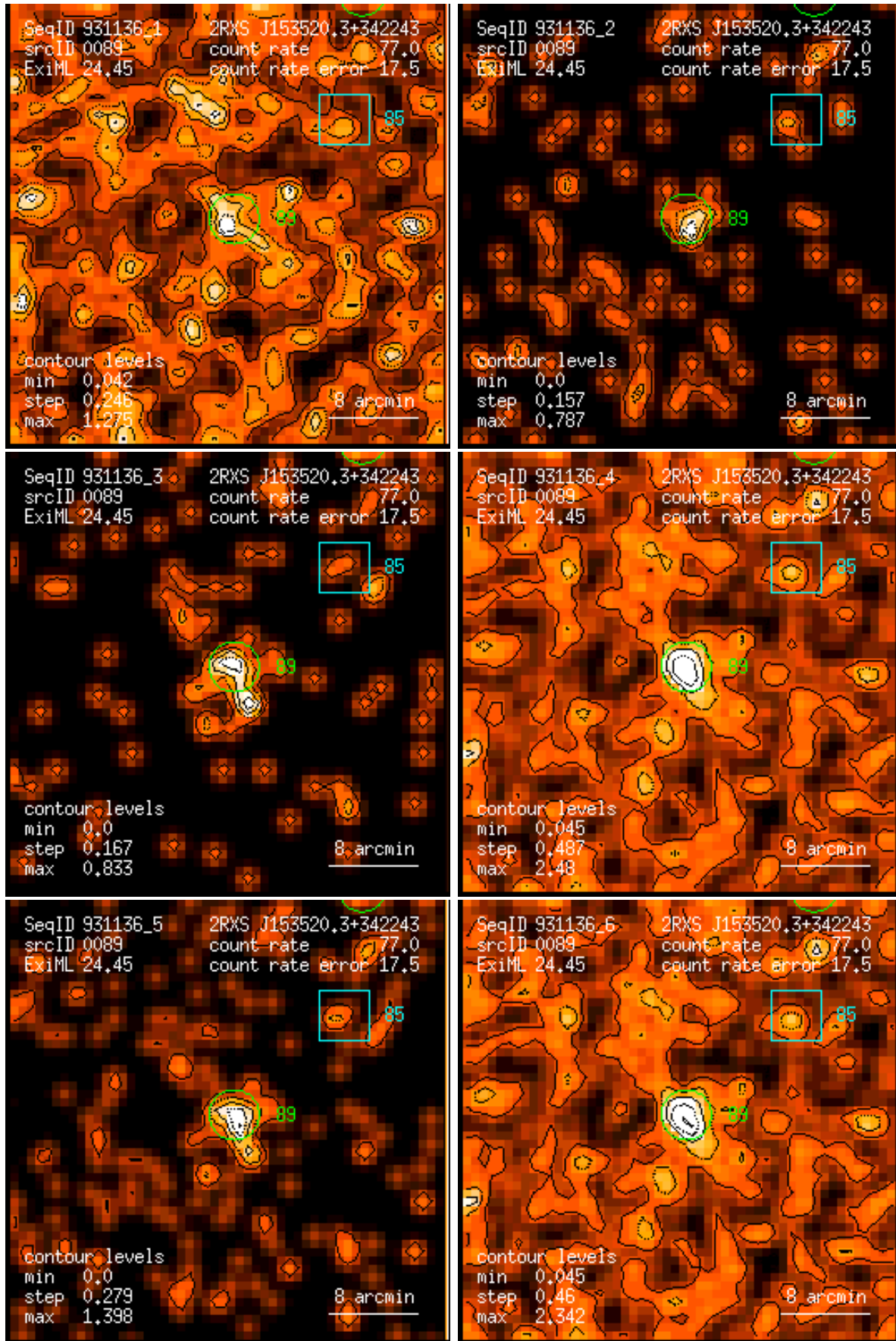
Figure 89: RASS 931136: detection 0089: band rate images, Gaussian filter: (1) PSPC channels 11 – 41, (2) 52 – 90, (3) 91 – 201, (4) 11 – 235, (5) 52 – 201, (6) 11 – 201. Broad band rates in counts/ks. Band rate contour levels in counts/ks/arcmin 2 .
