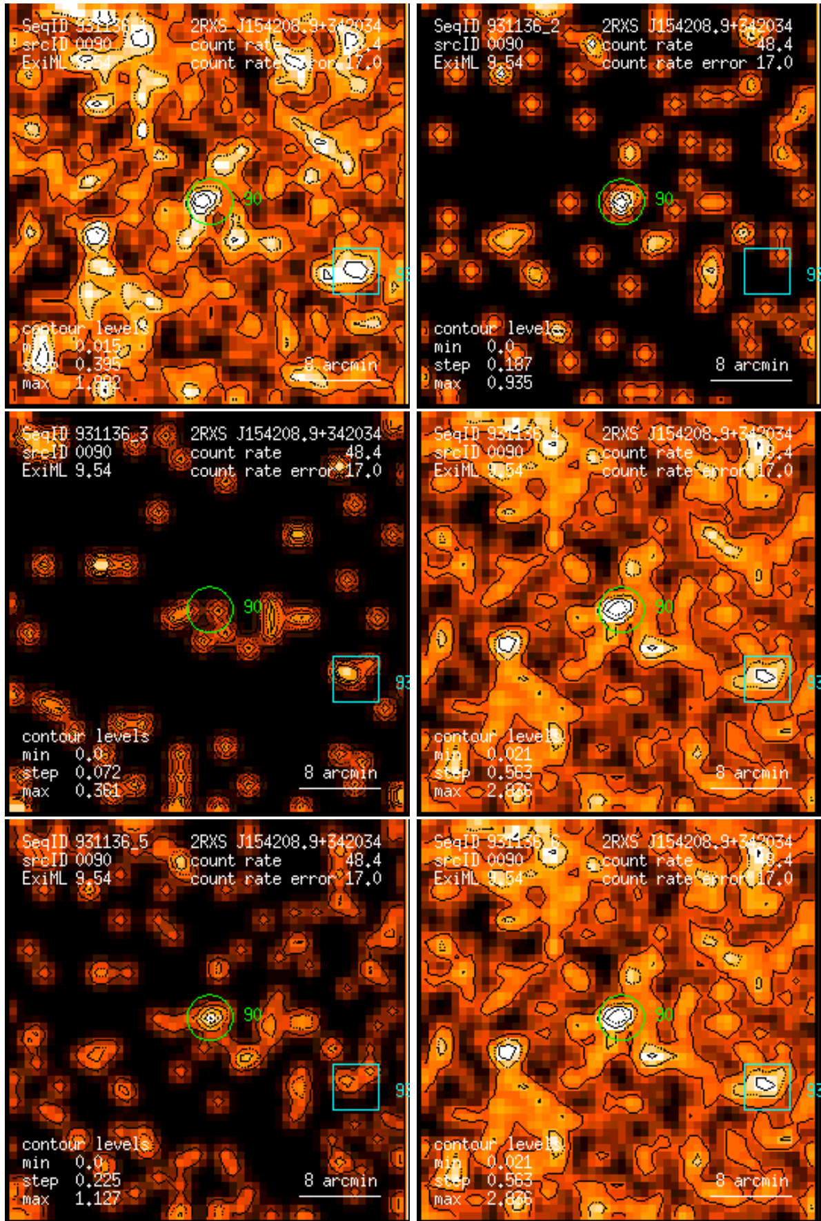
Figure 90: RASS 931136: detection 0090: band rate images, Gaussian filter: (1) PSPC channels 11 – 41, (2) 52 – 90, (3) 91 – 201, (4) 11 – 235, (5) 52 – 201, (6) 11 – 201. Broad band rates in counts/ks. Band rate contour levels in counts/ks/arcmin 2 .
