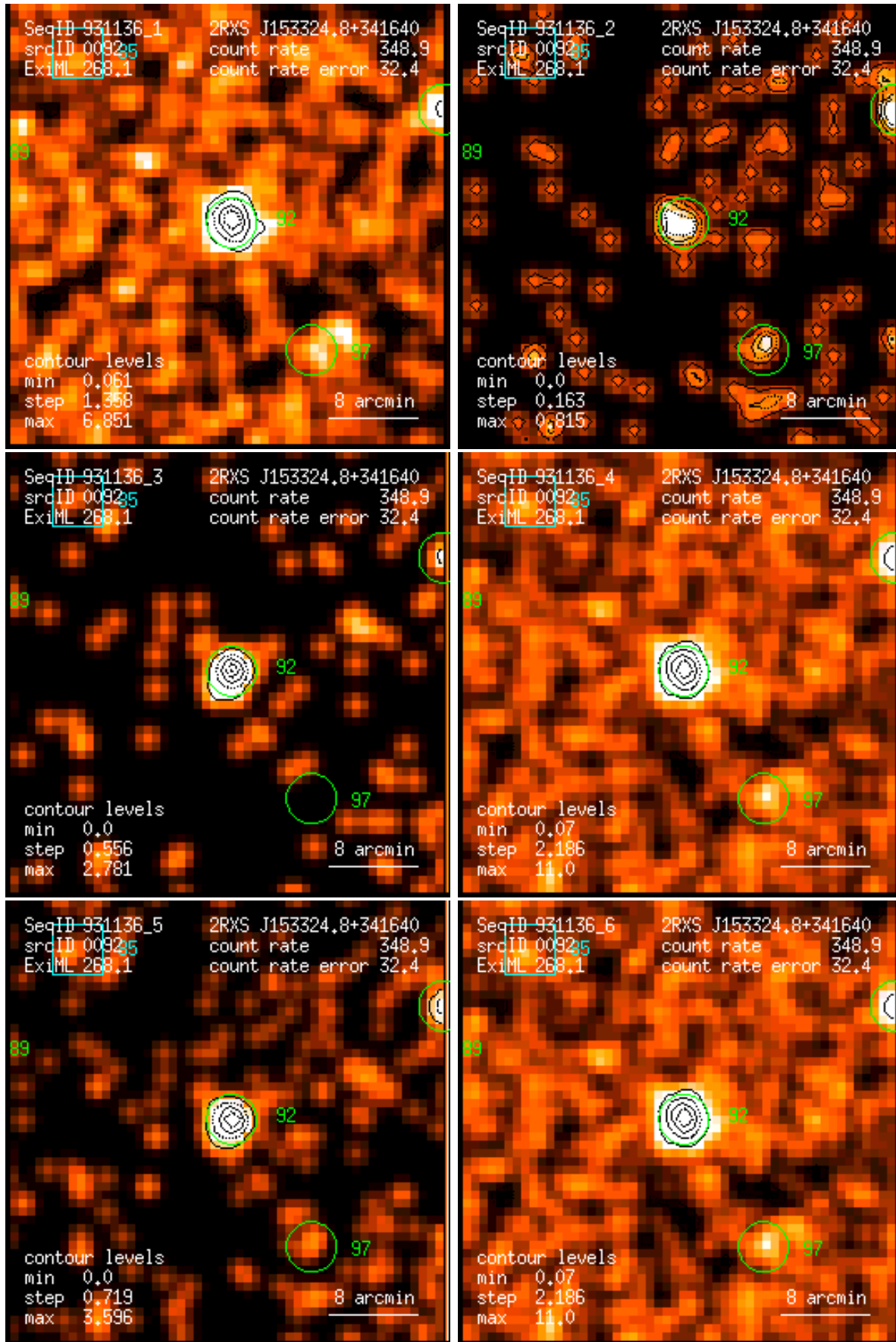
Figure 92: RASS 931136: detection 0092: band rate images, Gaussian filter: (1) PSPC channels 11 – 41, (2) 52 – 90, (3) 91 – 201, (4) 11 – 235, (5) 52 – 201, (6) 11 – 201. Broad band rates in counts/ks. Band rate contour levels in counts/ks/arcmin 2 .
