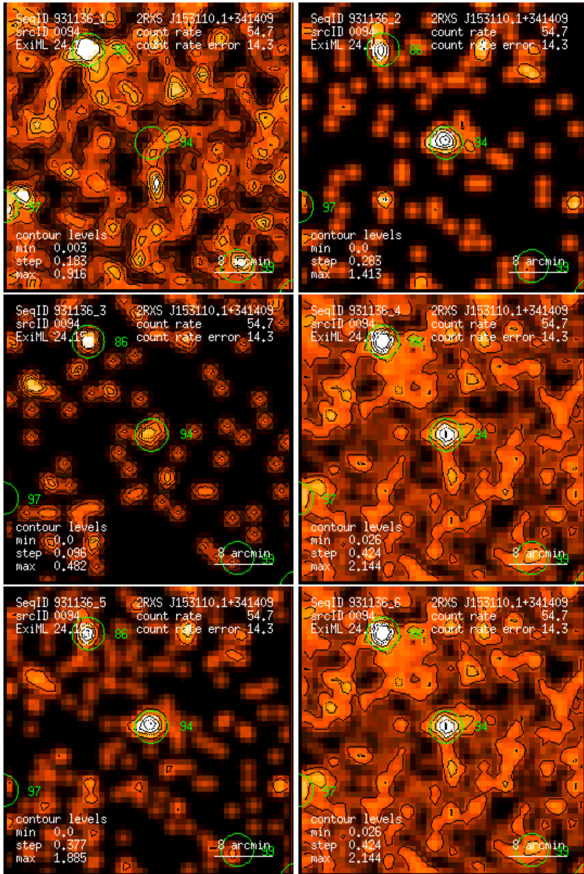
Figure 94: RASS 931136: detection 0094: band rate images, Gaussian filter: (1) PSPC channels 11 – 41, (2) 52 – 90, (3) 91 – 201, (4) 11 – 235, (5) 52 – 201, (6) 11 – 201. Broad band rates in counts/ks. Band rate contour levels in counts/ks/arcmin 2 .
