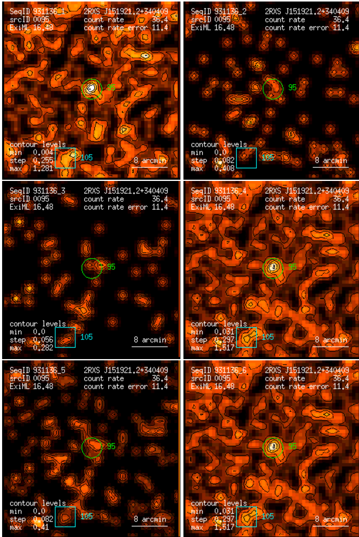
Figure 95: RASS 931136: detection 0095: band rate images, Gaussian filter: (1) PSPC channels 11 – 41, (2) 52 – 90, (3) 91 – 201, (4) 11 – 235, (5) 52 – 201, (6) 11 – 201. Broad band rates in counts/ks. Band rate contour levels in counts/ks/arcmin 2 .
