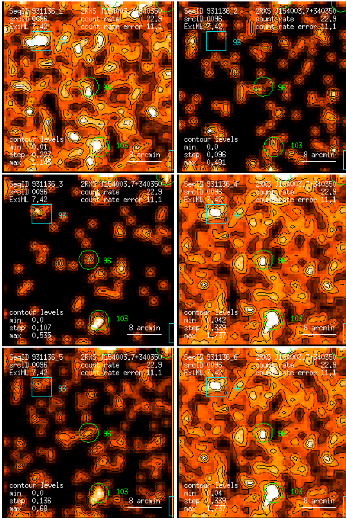
Figure 96: RASS 931136: detection 0096: band rate images, Gaussian filter: (1) PSPC channels 11 – 41, (2) 52 – 90, (3) 91 – 201, (4) 11 – 235, (5) 52 – 201, (6) 11 – 201. Broad band rates in counts/ks. Band rate contour levels in counts/ks/arcmin 2 .
