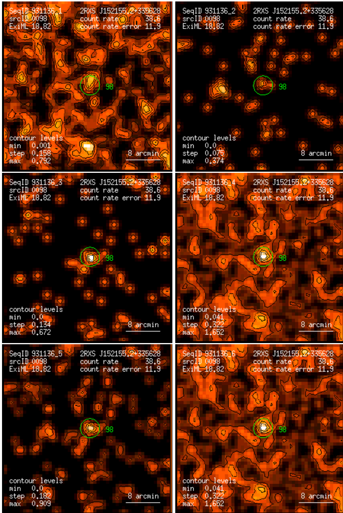
Figure 98: RASS 931136: detection 0098: band rate images, Gaussian filter: (1) PSPC channels 11 – 41, (2) 52 – 90, (3) 91 – 201, (4) 11 – 235, (5) 52 – 201, (6) 11 – 201. Broad band rates in counts/ks. Band rate contour levels in counts/ks/arcmin 2 .
