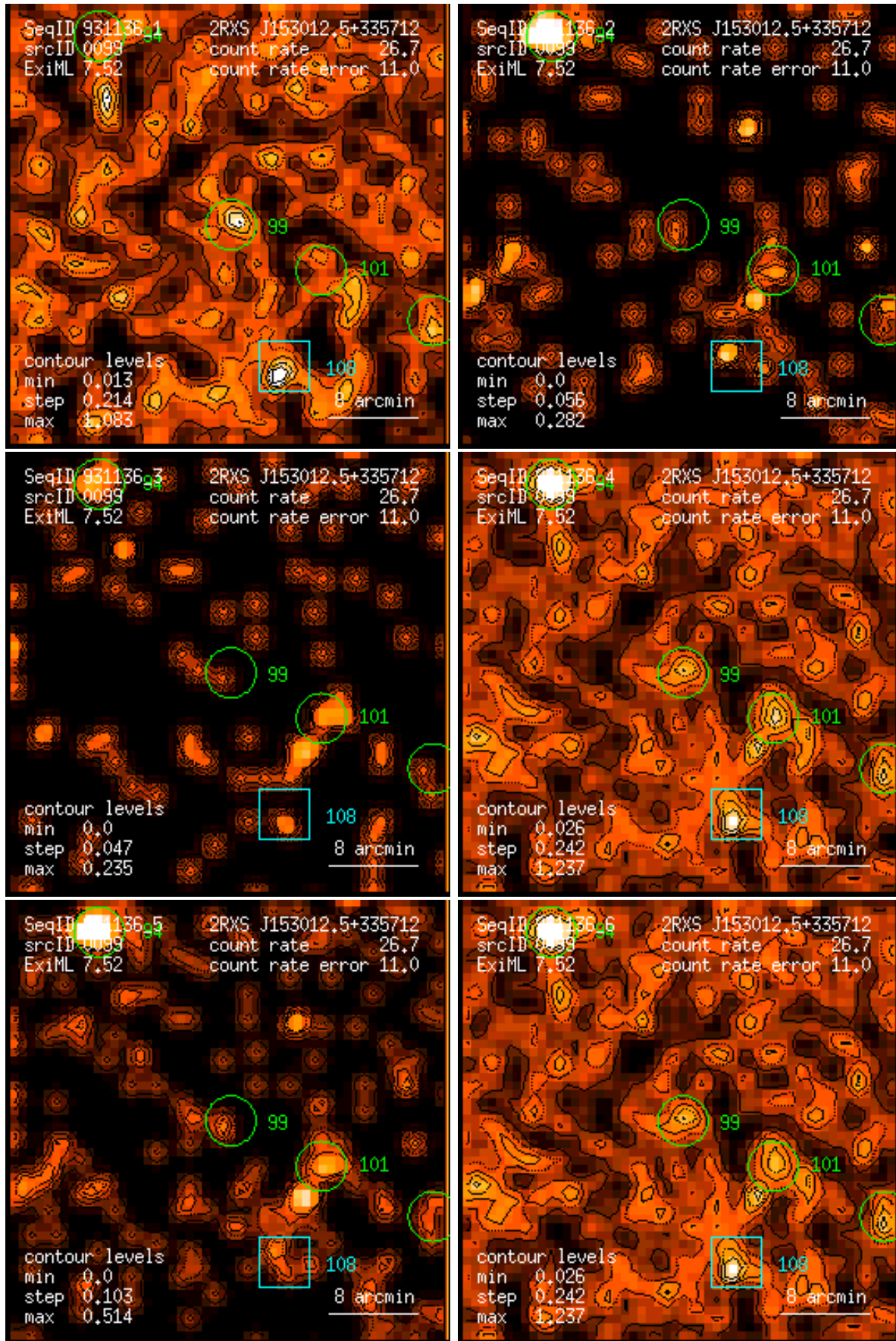
Figure 99: RASS 931136: detection 0099: band rate images, Gaussian filter: (1) PSPC channels 11 – 41, (2) 52 – 90, (3) 91 – 201, (4) 11 – 235, (5) 52 – 201, (6) 11 – 201. Broad band rates in counts/ks. Band rate contour levels in counts/ks/arcmin 2 .
