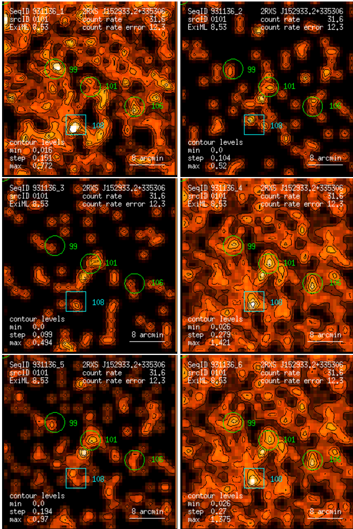
Figure 101: RASS 931136: detection 0101: band rate images, Gaussian filter: (1) PSPC channels 11 – 41, (2) 52 – 90, (3) 91 – 201, (4) 11 – 235, (5) 52 – 201, (6) 11 – 201. Broad band rates in counts/ks. Band rate contour levels in counts/ks/arcmin 2 .
