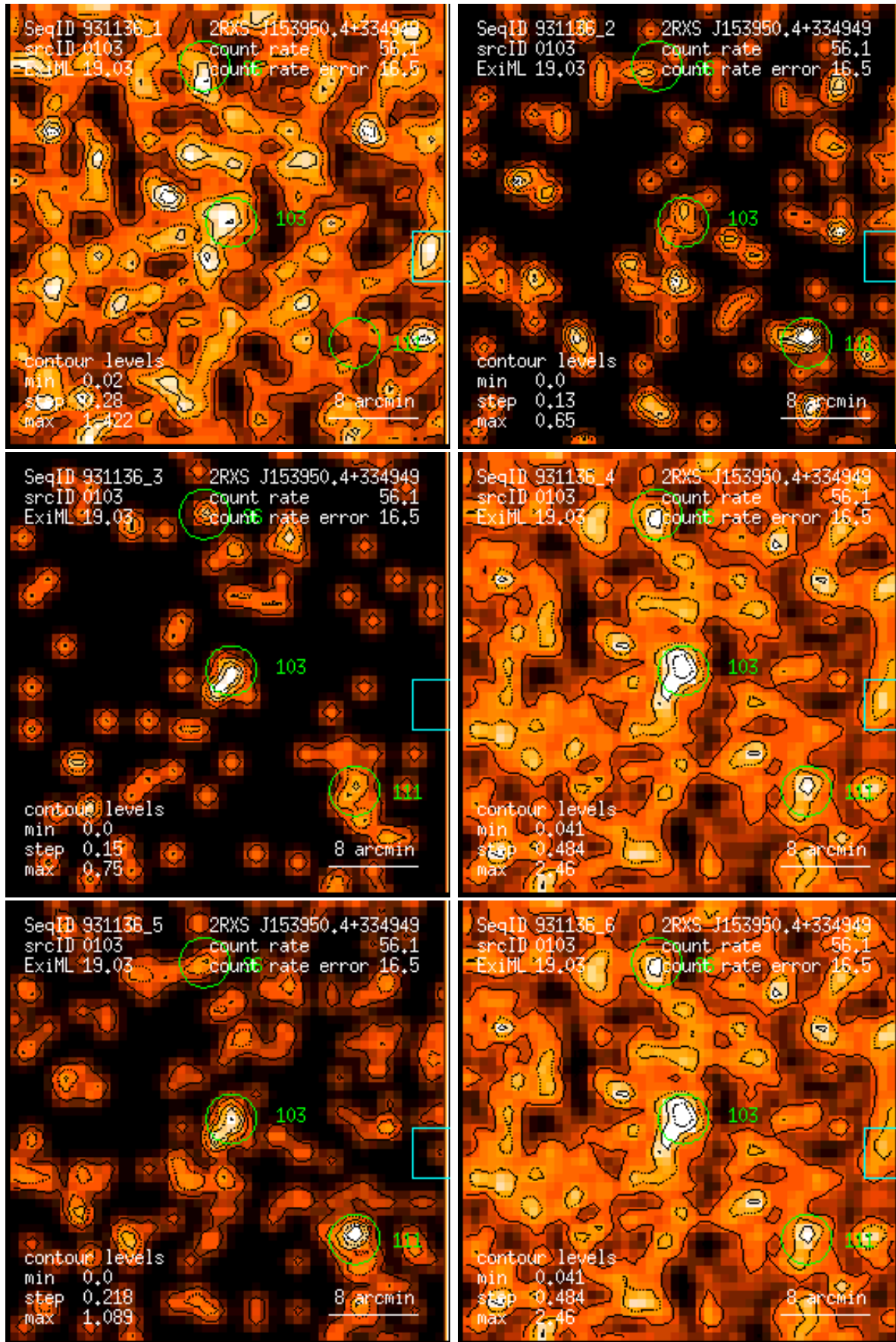
Figure 103: RASS 931136: detection 0103: band rate images, Gaussian filter: (1) PSPC channels 11 – 41, (2) 52 – 90, (3) 91 – 201, (4) 11 – 235, (5) 52 – 201, (6) 11 – 201. Broad band rates in counts/ks. Band rate contour levels in counts/ks/arcmin 2 .
