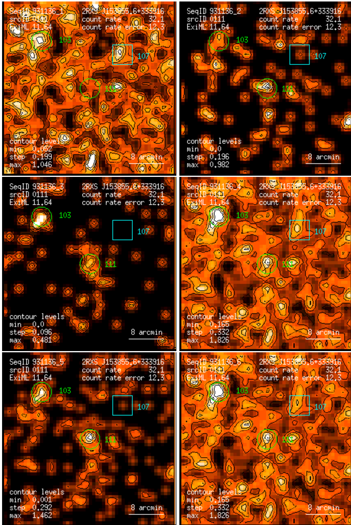
Figure 111: RASS 931136: detection 0111: band rate images, Gaussian filter: (1) PSPC channels 11 – 41, (2) 52 – 90, (3) 91 – 201, (4) 11 – 235, (5) 52 – 201, (6) 11 – 201. Broad band rates in counts/ks. Band rate contour levels in counts/ks/arcmin 2 .
