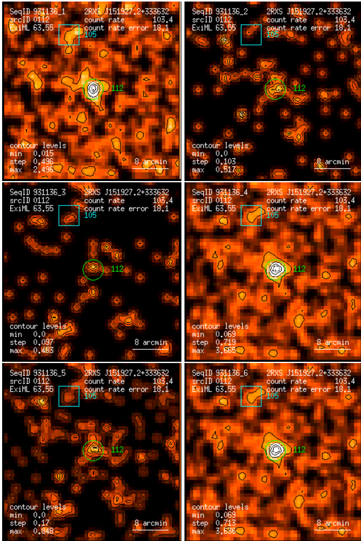
Figure 112: RASS 931136: detection 0112: band rate images, Gaussian filter: (1) PSPC channels 11 – 41, (2) 52 – 90, (3) 91 – 201, (4) 11 – 235, (5) 52 – 201, (6) 11 – 201. Broad band rates in counts/ks. Band rate contour levels in counts/ks/arcmin 2 .
