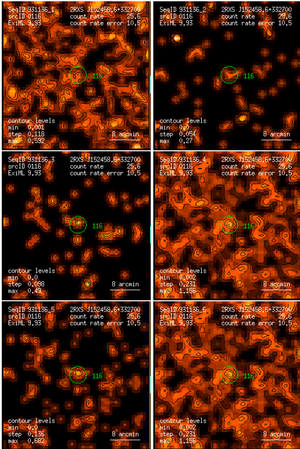
Figure 116: RASS 931136: detection 0116: band rate images, Gaussian filter: (1) PSPC channels 11 – 41, (2) 52 – 90, (3) 91 – 201, (4) 11 – 235, (5) 52 – 201, (6) 11 – 201. Broad band rates in counts/ks. Band rate contour levels in counts/ks/arcmin 2 .
