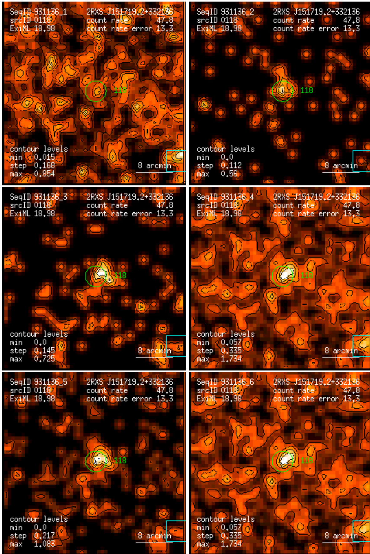
Figure 118: RASS 931136: detection 0118: band rate images, Gaussian filter: (1) PSPC channels 11 – 41, (2) 52 – 90, (3) 91 – 201, (4) 11 – 235, (5) 52 – 201, (6) 11 – 201. Broad band rates in counts/ks. Band rate contour levels in counts/ks/arcmin 2 .
