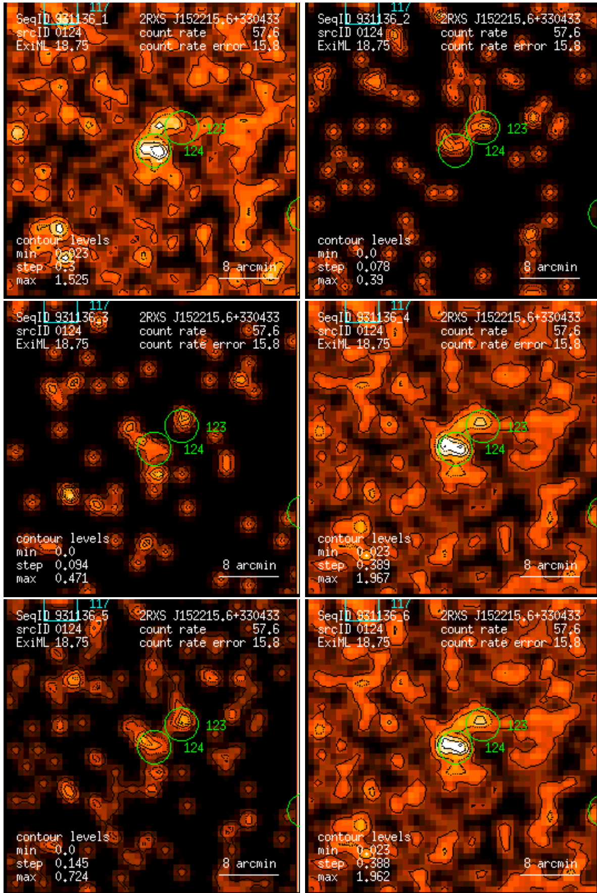
Figure 124: RASS 931136: detection 0124: band rate images, Gaussian filter: (1) PSPC channels 11 – 41, (2) 52 – 90, (3) 91 – 201, (4) 11 – 235, (5) 52 – 201, (6) 11 – 201. Broad band rates in counts/ks. Band rate contour levels in counts/ks/arcmin 2 .
