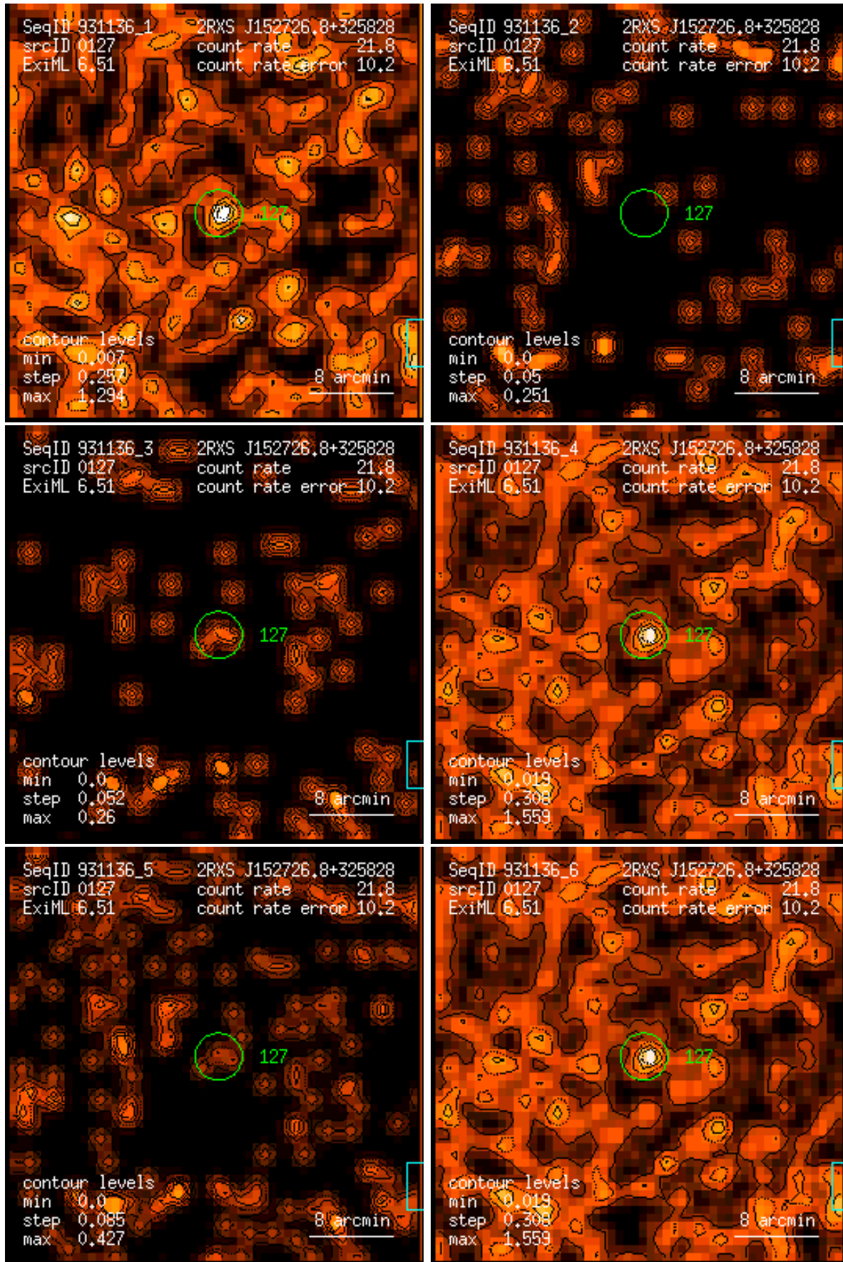
Figure 127: RASS 931136: detection 0127: band rate images, Gaussian filter: (1) PSPC channels 11 – 41, (2) 52 – 90, (3) 91 – 201, (4) 11 – 235, (5) 52 – 201, (6) 11 – 201. Broad band rates in counts/ks. Band rate contour levels in counts/ks/arcmin 2 .
