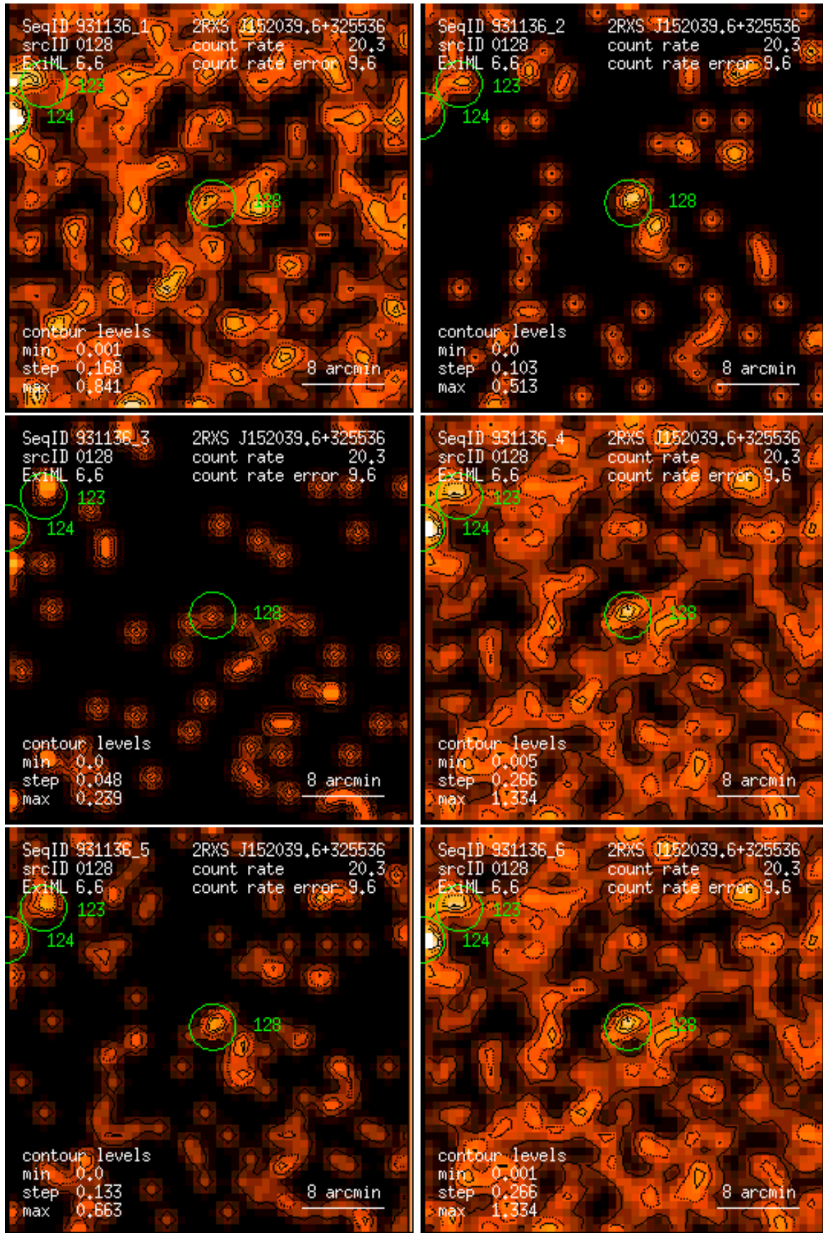
Figure 128: RASS 931136: detection 0128: band rate images, Gaussian filter: (1) PSPC channels 11 – 41, (2) 52 – 90, (3) 91 – 201, (4) 11 – 235, (5) 52 – 201, (6) 11 – 201. Broad band rates in counts/ks. Band rate contour levels in counts/ks/arcmin 2 .
