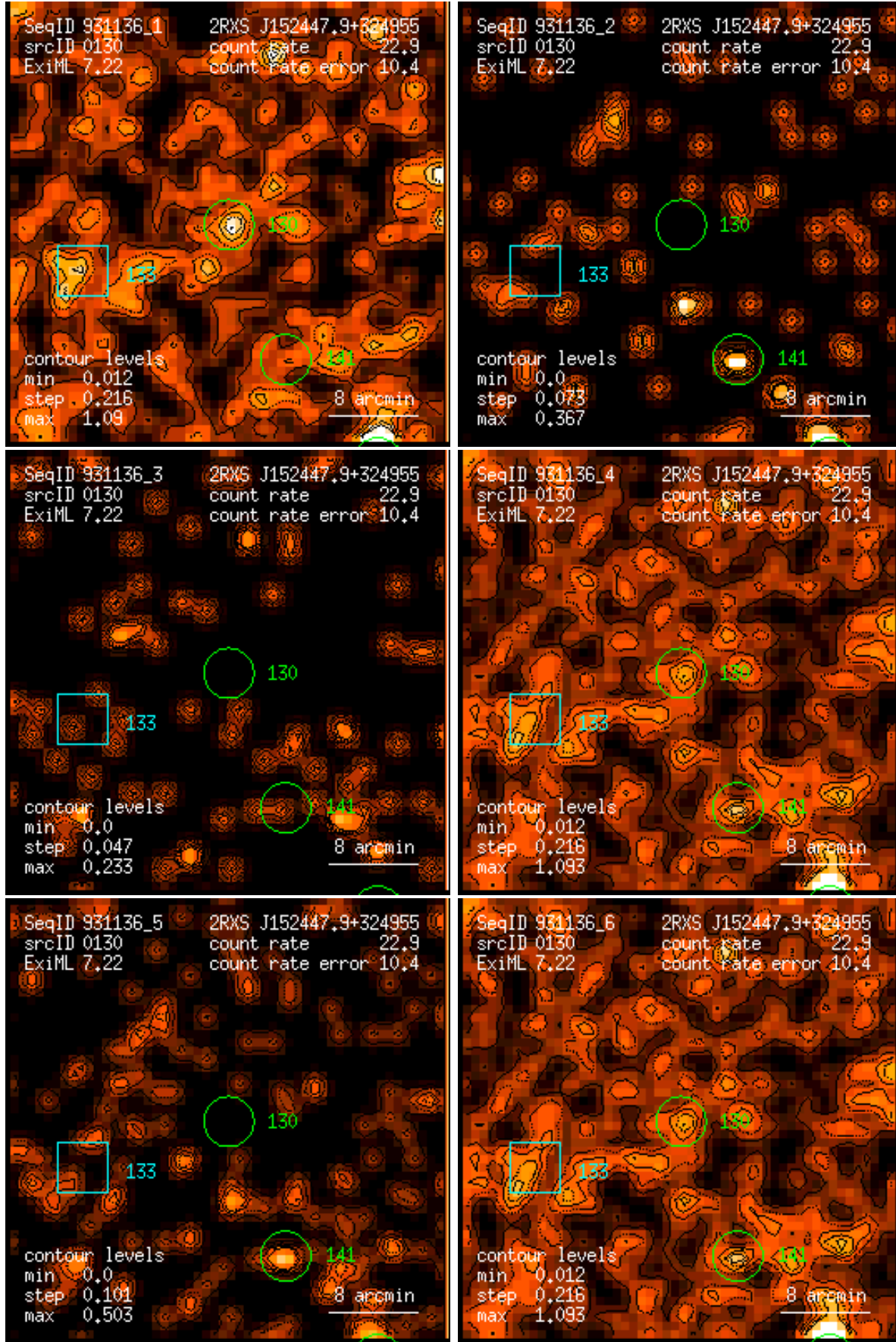
Figure 130: RASS 931136: detection 0130: band rate images, Gaussian filter: (1) PSPC channels 11 – 41, (2) 52 – 90, (3) 91 – 201, (4) 11 – 235, (5) 52 – 201, (6) 11 – 201. Broad band rates in counts/ks. Band rate contour levels in counts/ks/arcmin 2 .
