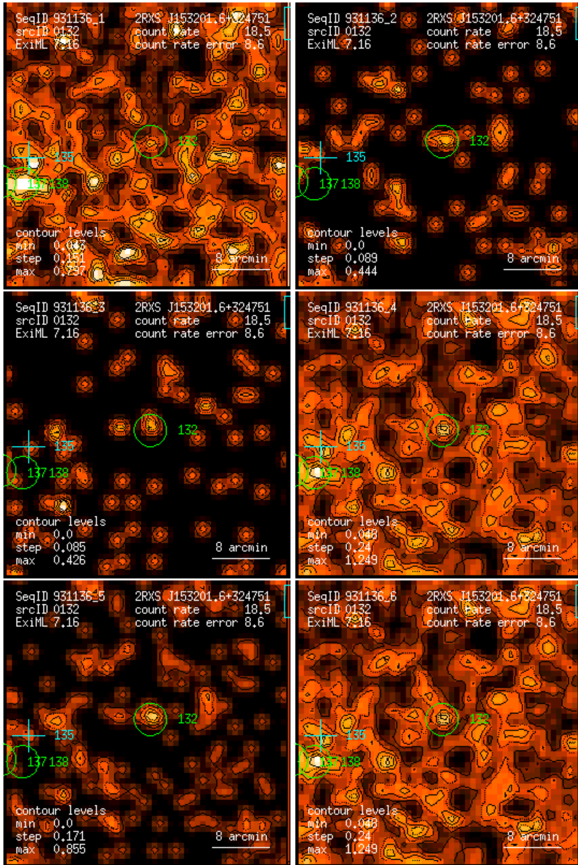
Figure 132: RASS 931136: detection 0132: band rate images, Gaussian filter: (1) PSPC channels 11 – 41, (2) 52 – 90, (3) 91 – 201, (4) 11 – 235, (5) 52 – 201, (6) 11 – 201. Broad band rates in counts/ks. Band rate contour levels in counts/ks/arcmin 2 .
