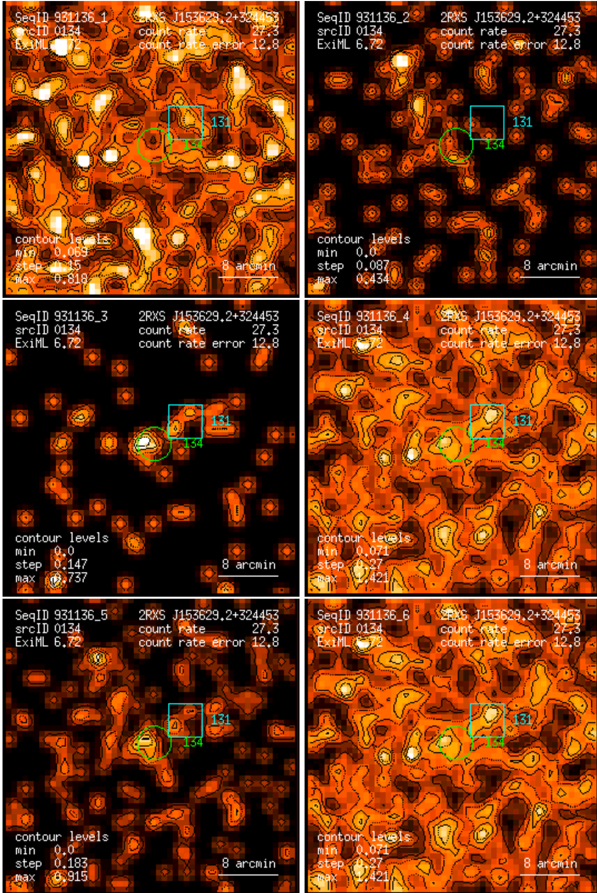
Figure 134: RASS 931136: detection 0134: band rate images, Gaussian filter: (1) PSPC channels 11 – 41, (2) 52 – 90, (3) 91 – 201, (4) 11 – 235, (5) 52 – 201, (6) 11 – 201. Broad band rates in counts/ks. Band rate contour levels in counts/ks/arcmin 2 .
