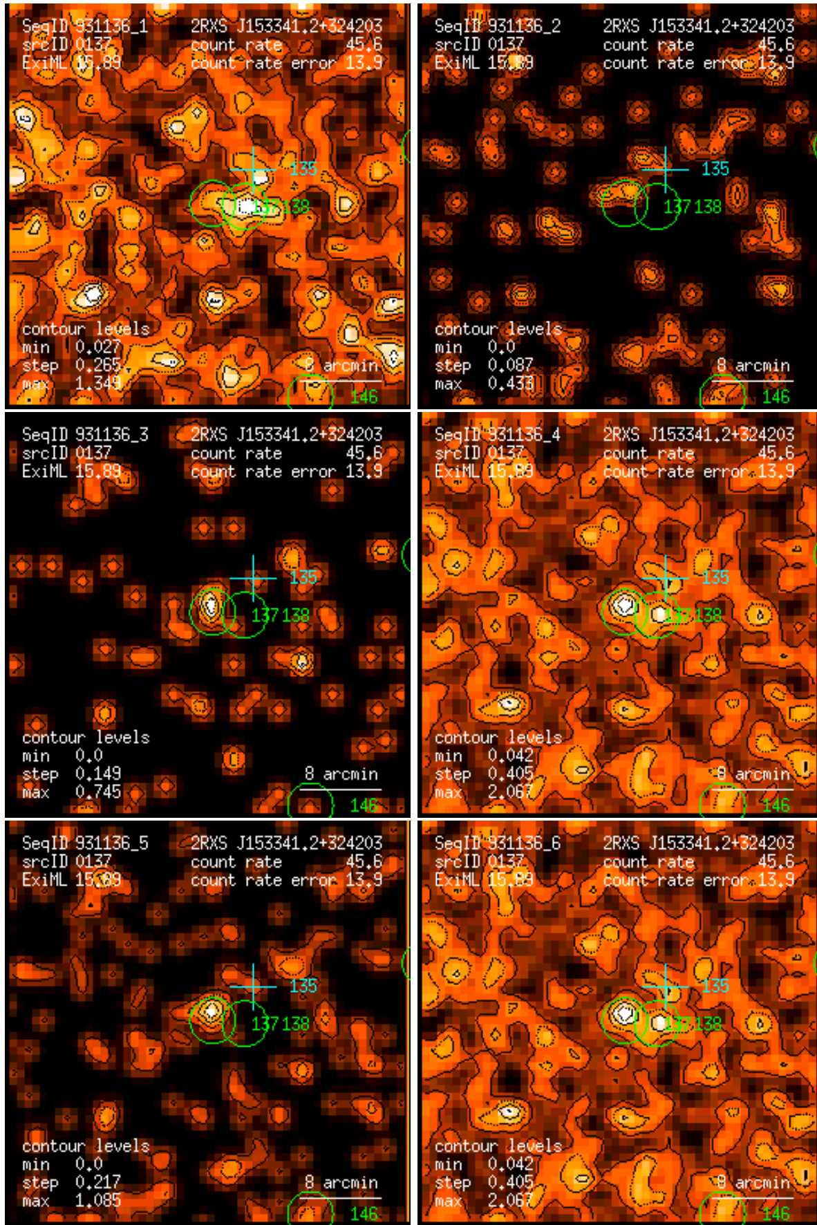
Figure 137: RASS 931136: detection 0137: band rate images, Gaussian filter: (1) PSPC channels 11 – 41, (2) 52 – 90, (3) 91 – 201, (4) 11 – 235, (5) 52 – 201, (6) 11 – 201. Broad band rates in counts/ks. Band rate contour levels in counts/ks/arcmin 2 .
