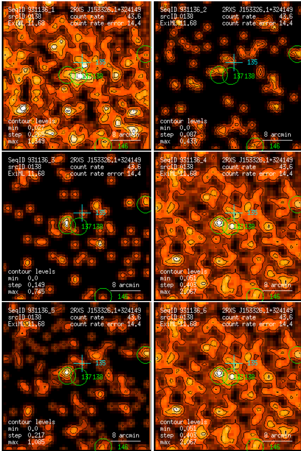
Figure 138: RASS 931136: detection 0138: band rate images, Gaussian filter: (1) PSPC channels 11 – 41, (2) 52 – 90, (3) 91 – 201, (4) 11 – 235, (5) 52 – 201, (6) 11 – 201. Broad band rates in counts/ks. Band rate contour levels in counts/ks/arcmin 2 .
