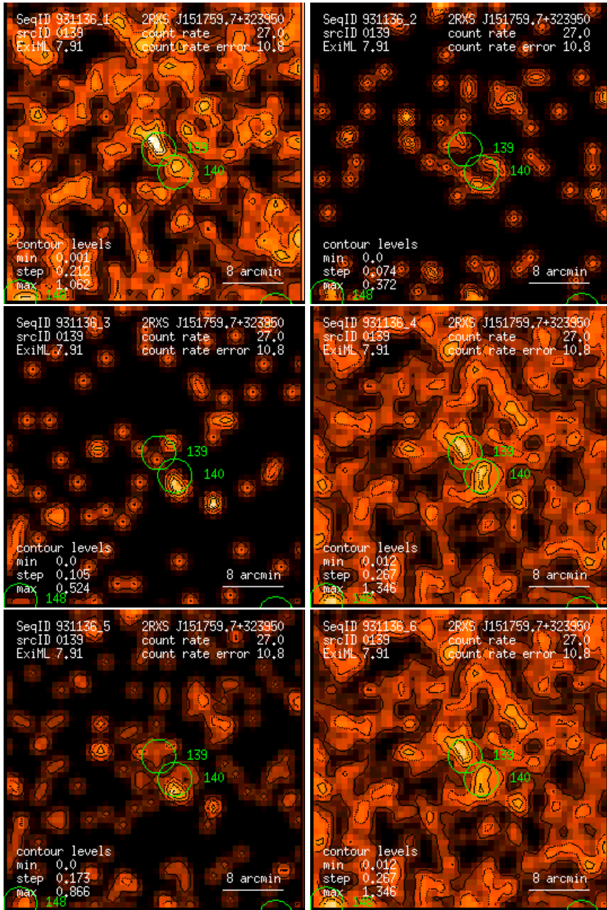
Figure 139: RASS 931136: detection 0139: band rate images, Gaussian filter: (1) PSPC channels 11 – 41, (2) 52 – 90, (3) 91 – 201, (4) 11 – 235, (5) 52 – 201, (6) 11 – 201. Broad band rates in counts/ks. Band rate contour levels in counts/ks/arcmin 2 .
