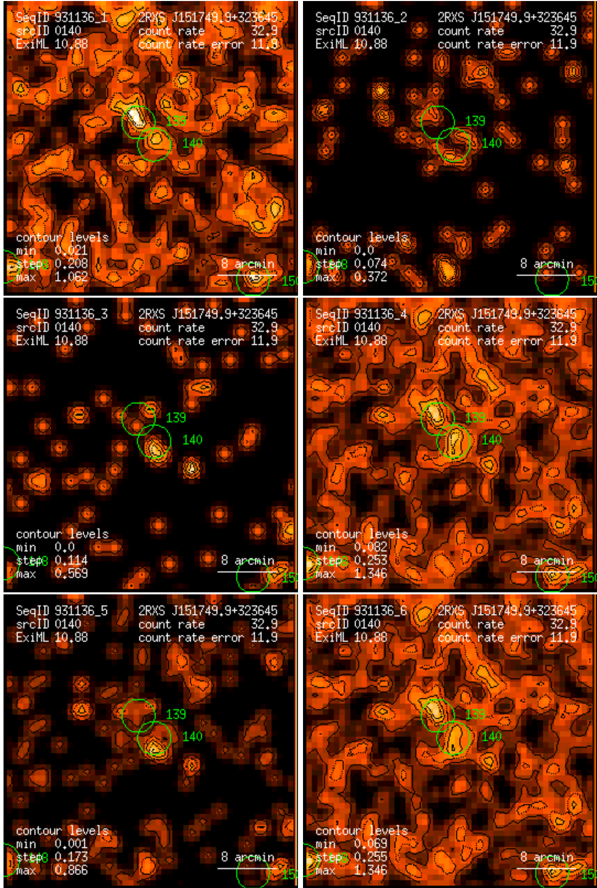
Figure 140: RASS 931136: detection 0140: band rate images, Gaussian filter: (1) PSPC channels 11 – 41, (2) 52 – 90, (3) 91 – 201, (4) 11 – 235, (5) 52 – 201, (6) 11 – 201. Broad band rates in counts/ks. Band rate contour levels in counts/ks/arcmin 2 .
