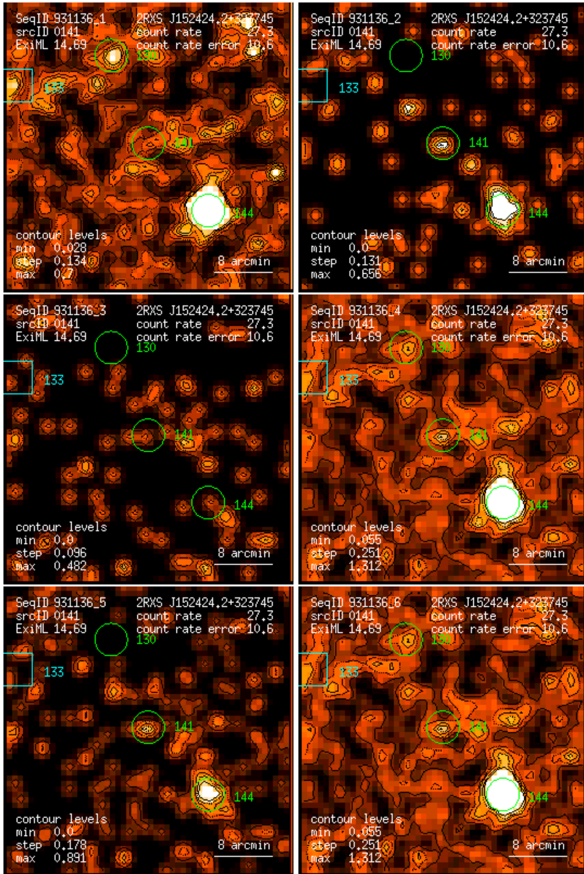
Figure 141: RASS 931136: detection 0141: band rate images, Gaussian filter: (1) PSPC channels 11 – 41, (2) 52 – 90, (3) 91 – 201, (4) 11 – 235, (5) 52 – 201, (6) 11 – 201. Broad band rates in counts/ks. Band rate contour levels in counts/ks/arcmin 2 .
