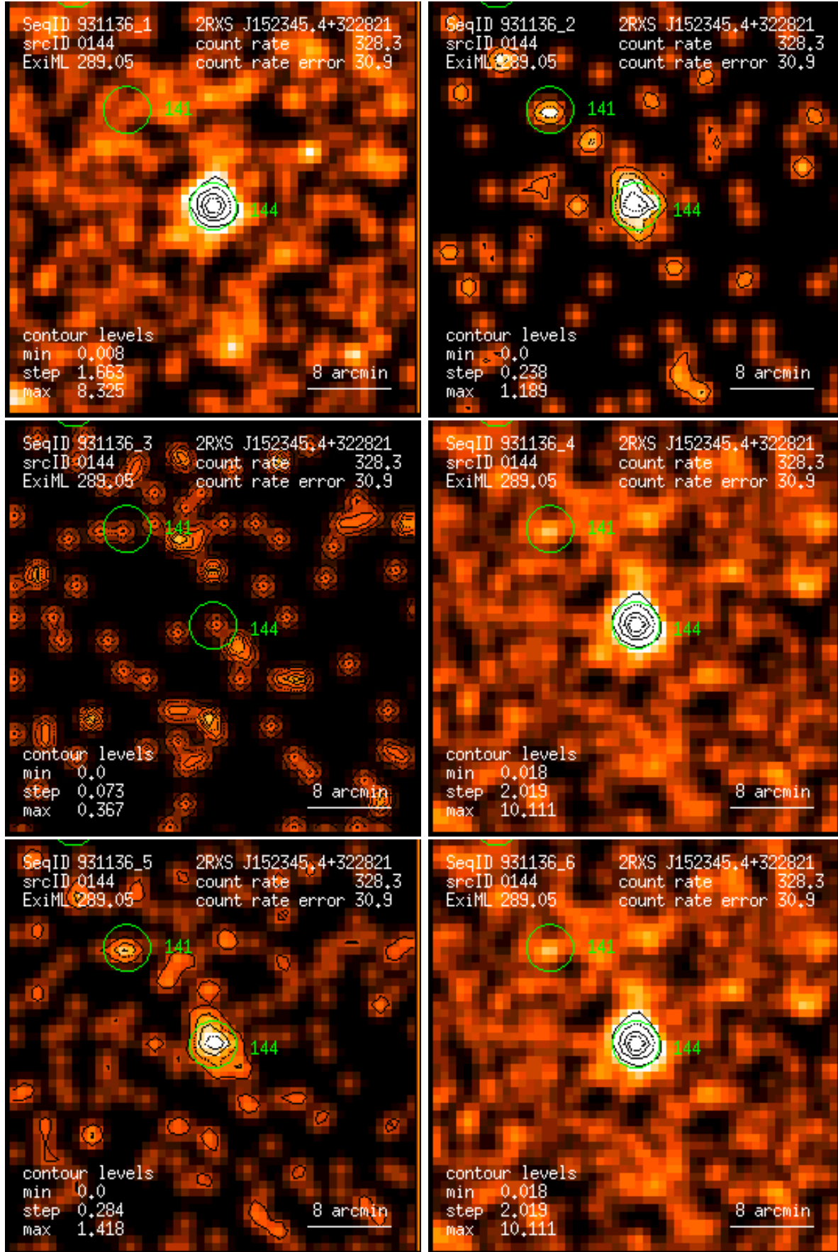
Figure 144: RASS 931136: detection 0144: band rate images, Gaussian filter: (1) PSPC channels 11 – 41, (2) 52 – 90, (3) 91 – 201, (4) 11 – 235, (5) 52 – 201, (6) 11 – 201. Broad band rates in counts/ks. Band rate contour levels in counts/ks/arcmin 2 .
