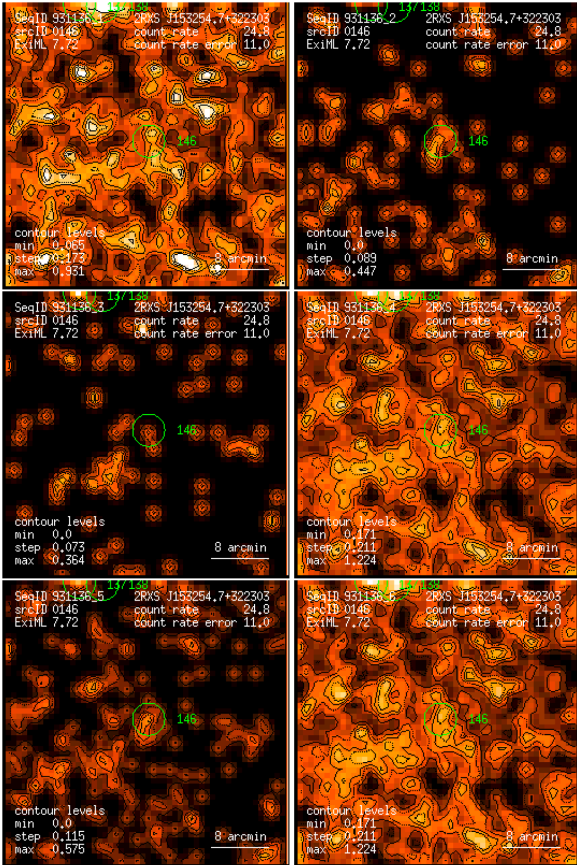
Figure 146: RASS 931136: detection 0146: band rate images, Gaussian filter: (1) PSPC channels 11 – 41, (2) 52 – 90, (3) 91 – 201, (4) 11 – 235, (5) 52 – 201, (6) 11 – 201. Broad band rates in counts/ks. Band rate contour levels in counts/ks/arcmin 2 .
